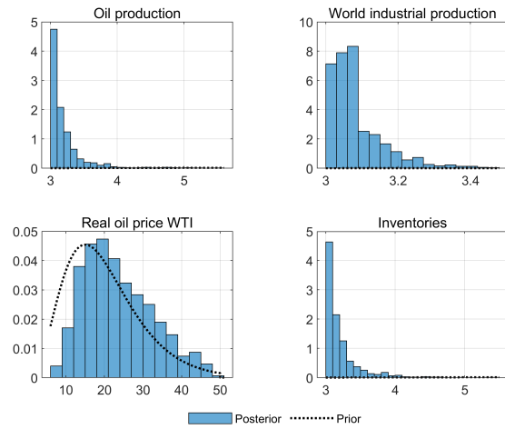
(a) t-Distribution
