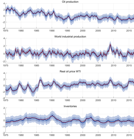
(a) SV
