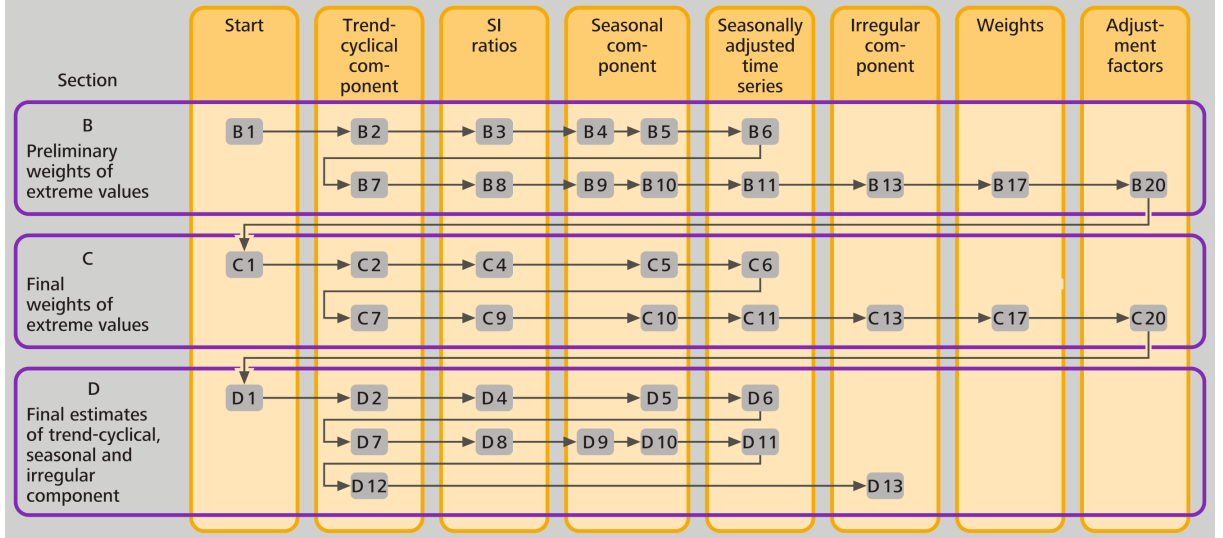
Figure 1: Basic workflow of the classical X-11 method as implemented in JDemetra+. Labels in grey boxes refer to the names of the X-11 output tables.
