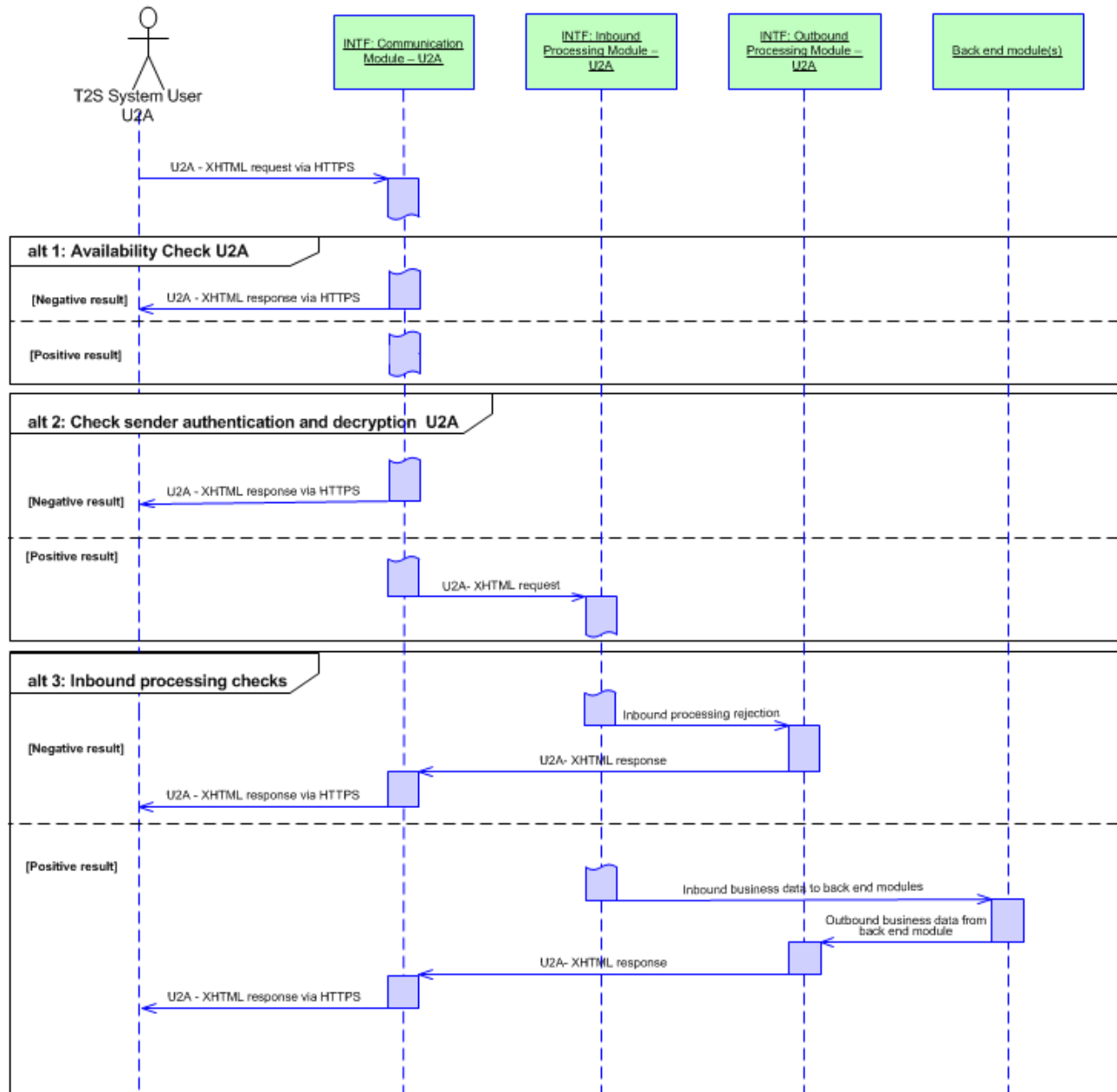
Figure 13: Interface via U2A
