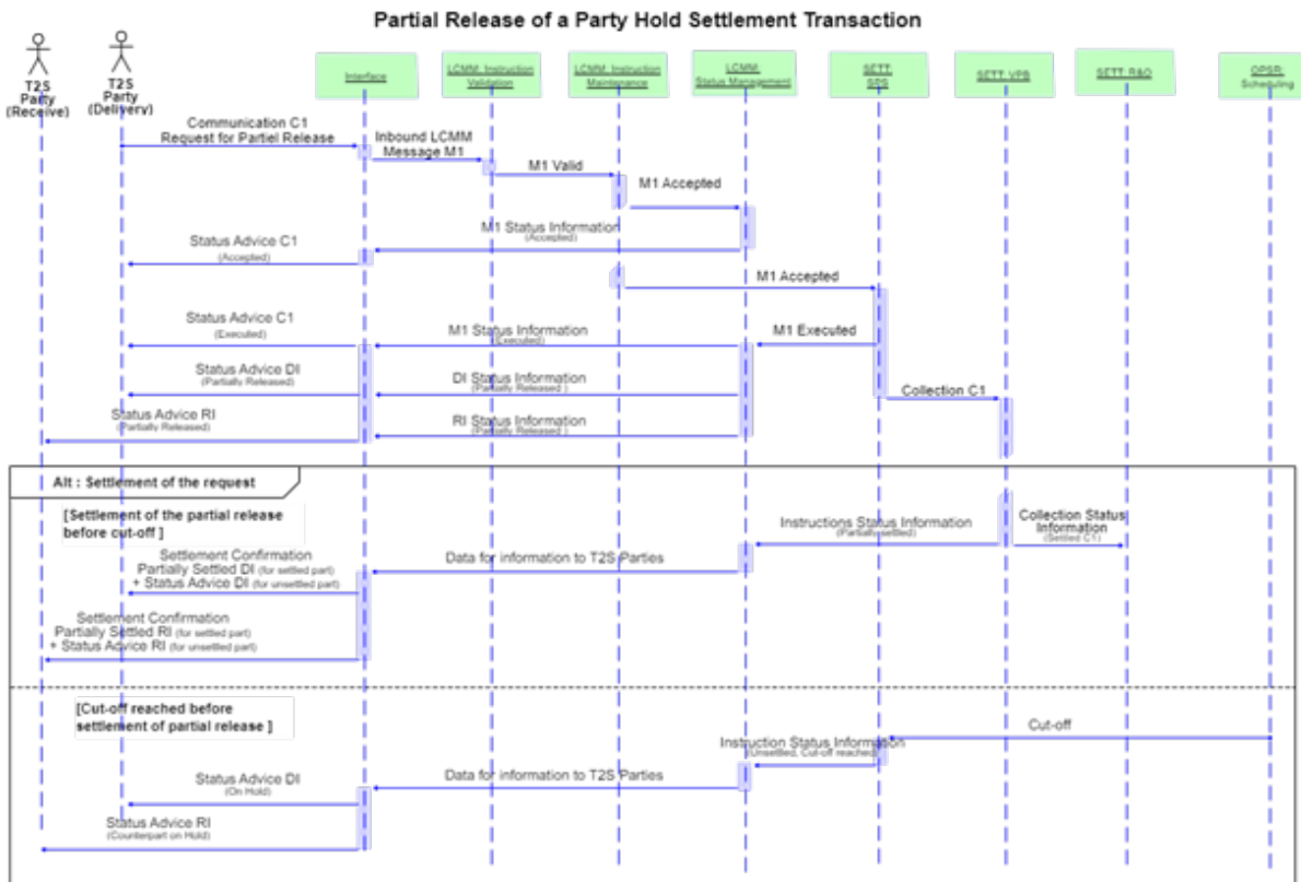
Figure 40: Settlement process Partial Party Hold Release
