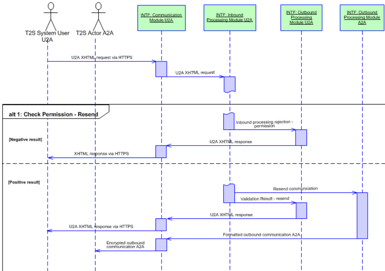
Figure 14: Interface via U2A - Resend
