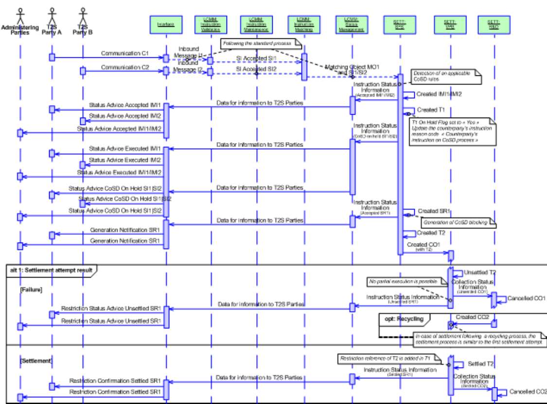
Figure 27: Settlement process for CoSD Activation
