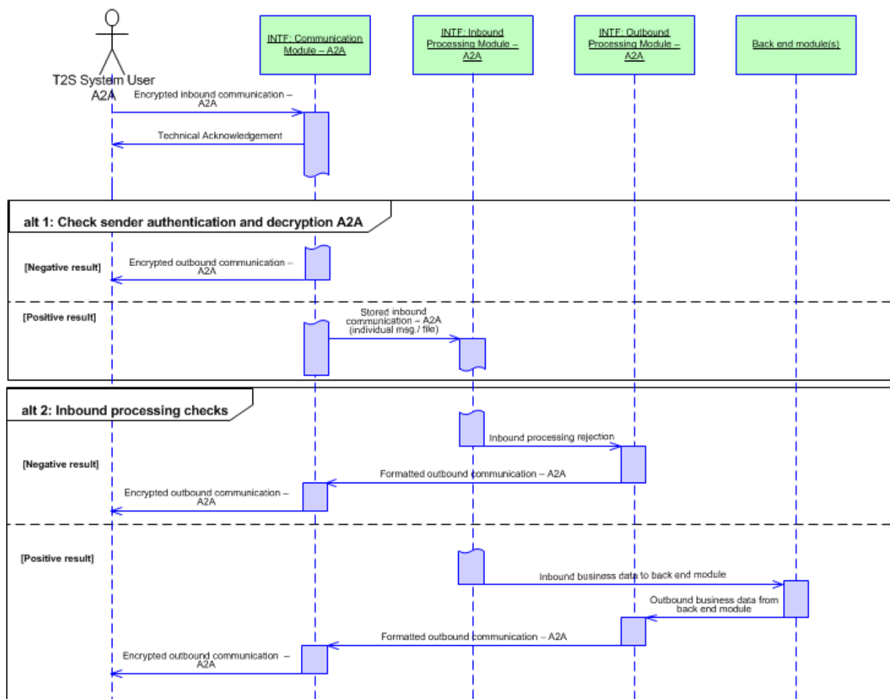
Figure 10: Interface via A2A
