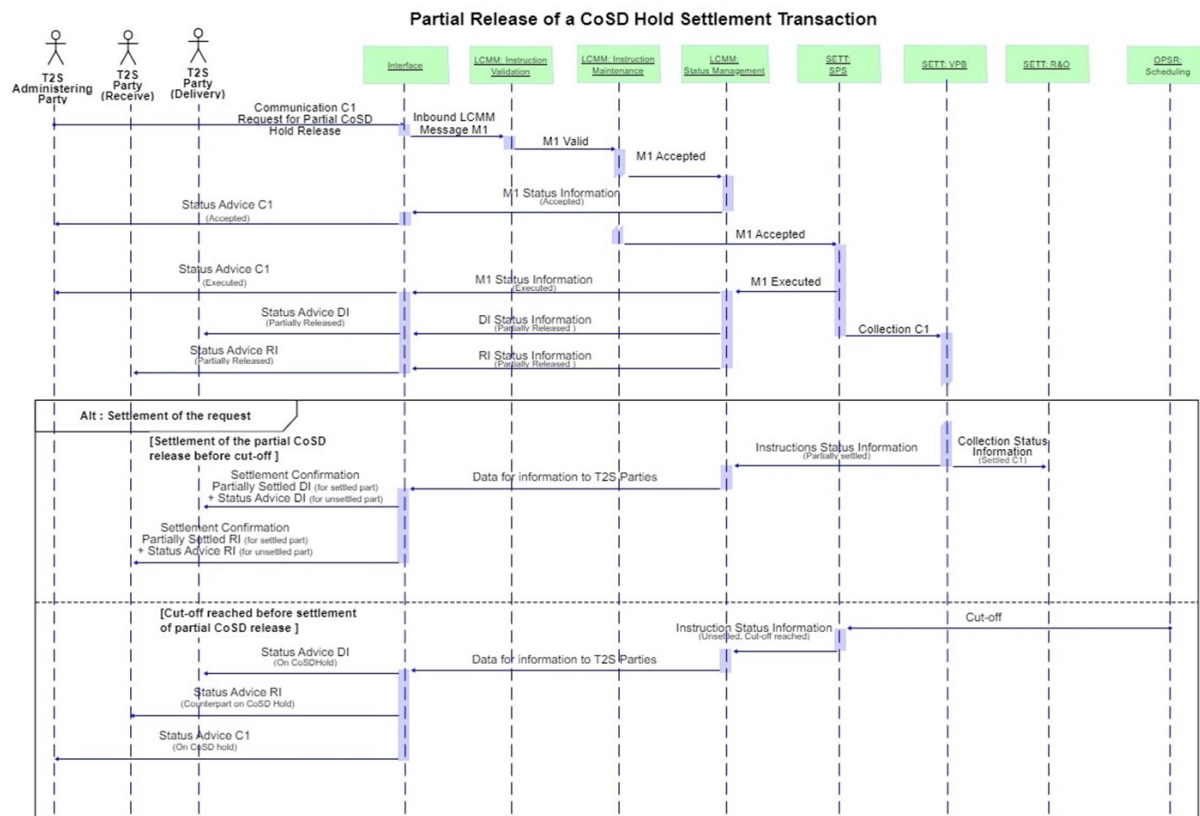
Figure 41: Settlement process Partial CoSD Release
