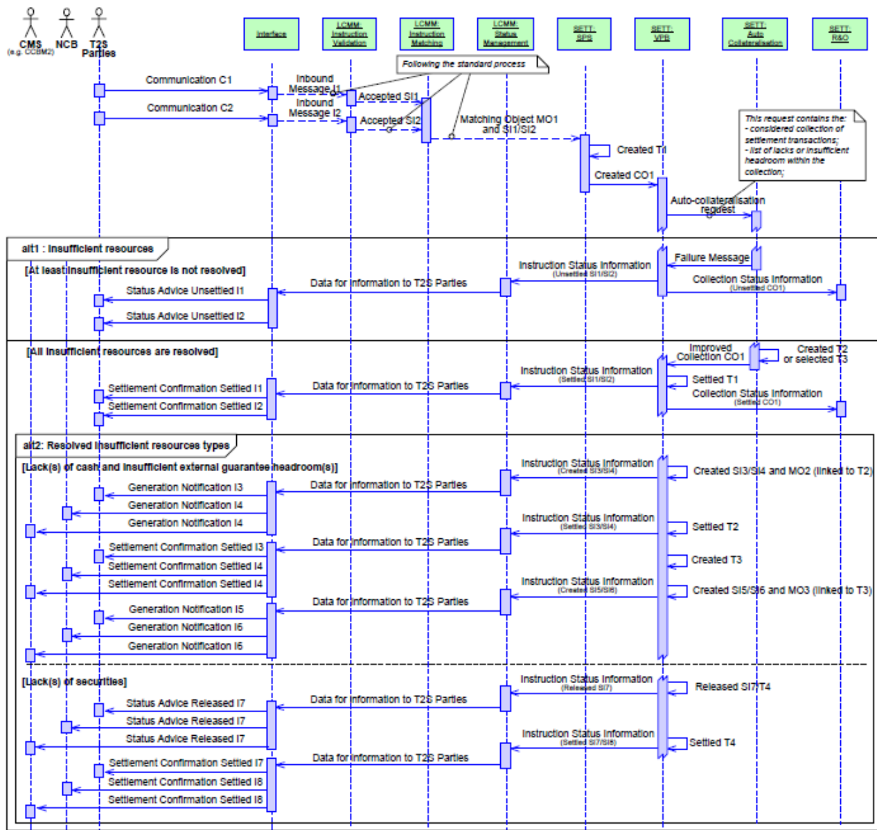
Figure 26: Settlement process with auto-collateralisation during booking process
