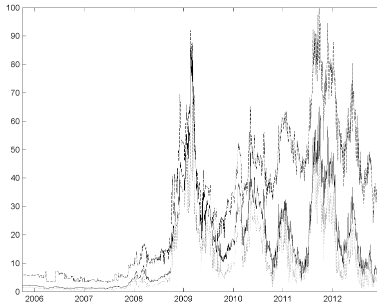
Figure 1: TERM STRUCTURE OF 1-YEAR, 5-YEAR AND 10-YEAR CDS SPREADS FOR GERMAN SOVEREIGN
