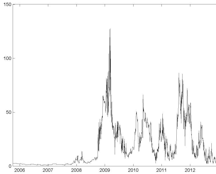
Figure 2: CDS-IMPLIED DEFAULT INTENSITY OF GERMAN SOVEREIGN
