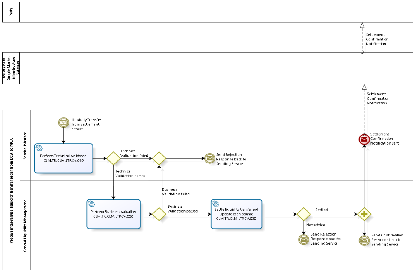
Business Process Model 2: Process inter-service liquidity transfer order from T2S/RTGS/TIPS Account to CLM Account
