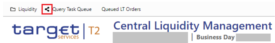
Figure 11: Shared Bookmark
