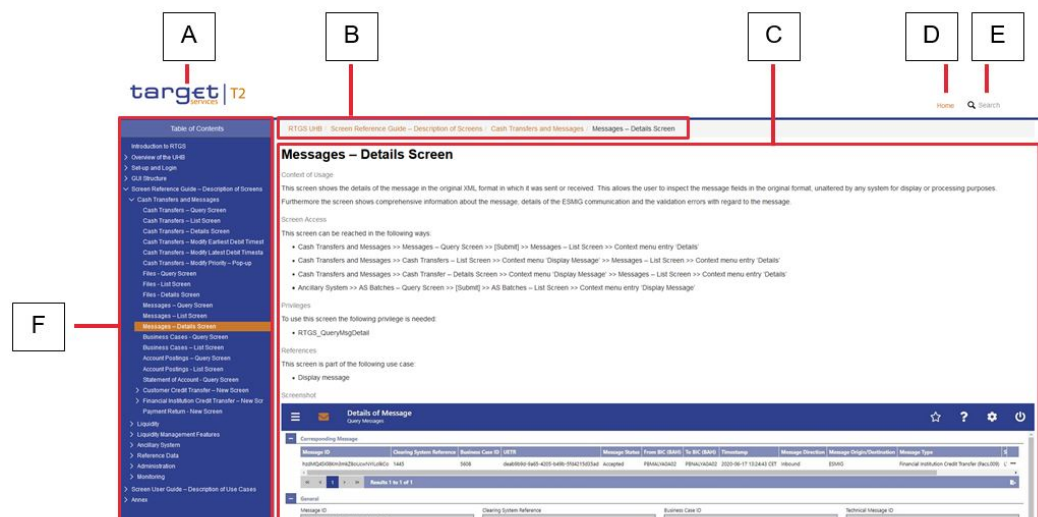
Figure 75: Online Help
