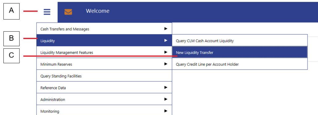
Figure 1: CLM Menu
