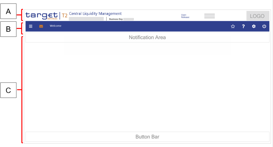
Figure 2: Screen Structure
