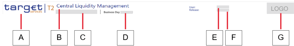
Figure 3: Header
