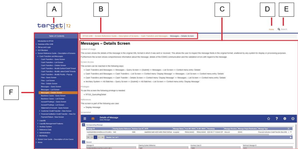
Figure 74: Online Help
