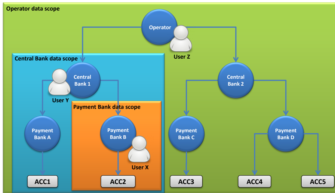
DIAGRAM 8 - DATA SCOPES
