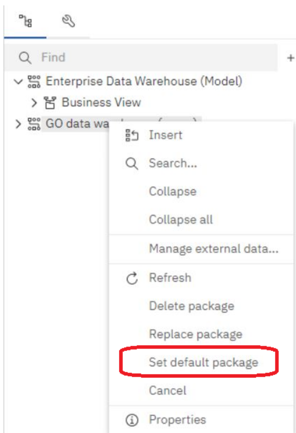
Figure 521: Adding data - Add a source - Right click item - Set default package
