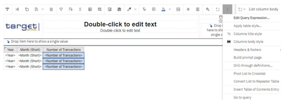
Figure 533: Change a list into a crosstab - More icon - Pivot List to Crosstab
