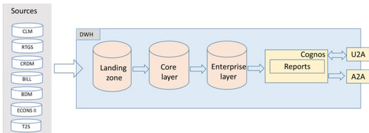
Figure 1: DWH high level overview
