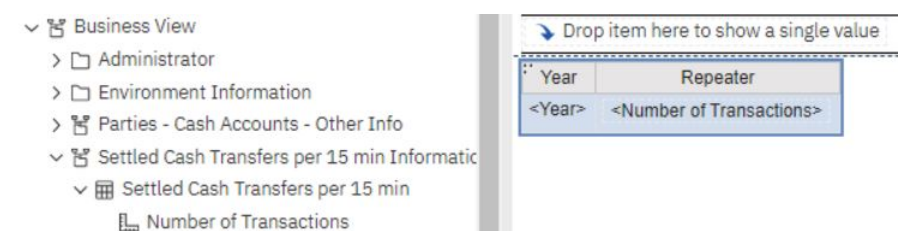
Figure 531: Using Repeaters - List with all Number of Transactions in a single row
