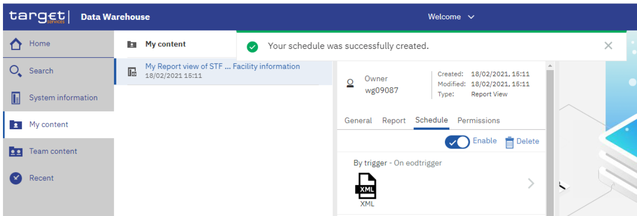
Figure 144: Welcome page - My content - Properties - Schedule
