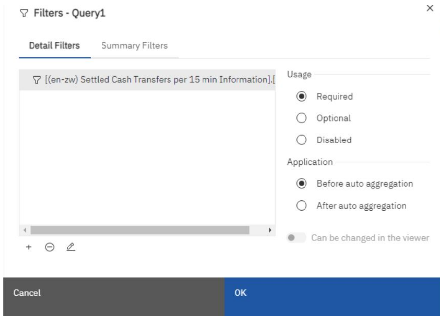
Figure 569: Modifying prompts - Filters - Usage box
