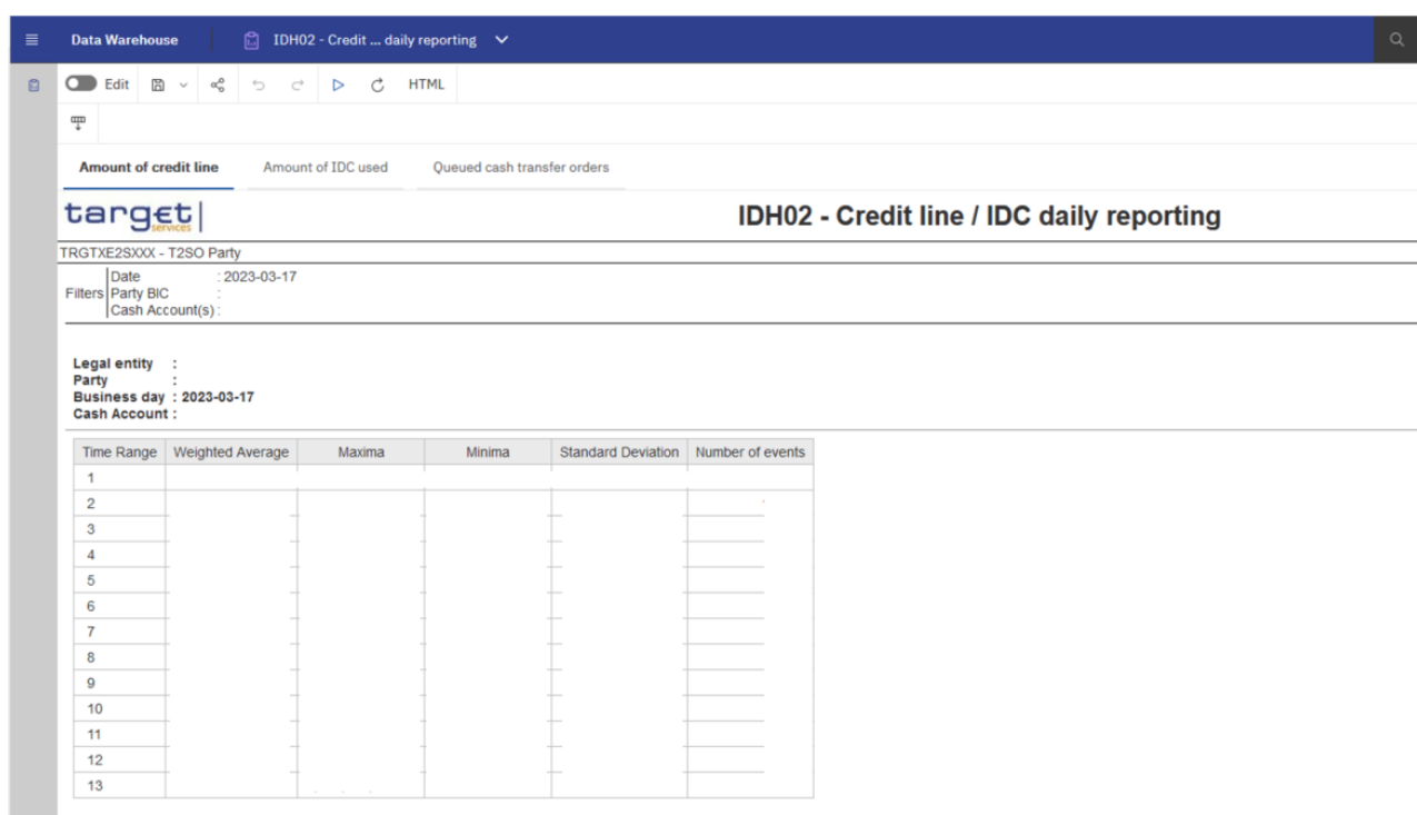
Figure 586: IDH02 Results screen (1) for credit line amounts
