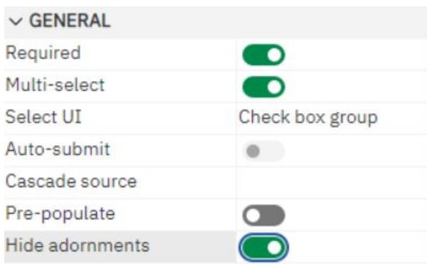
Figure 576: Modifying prompts - Properties - General - Hide adornments
