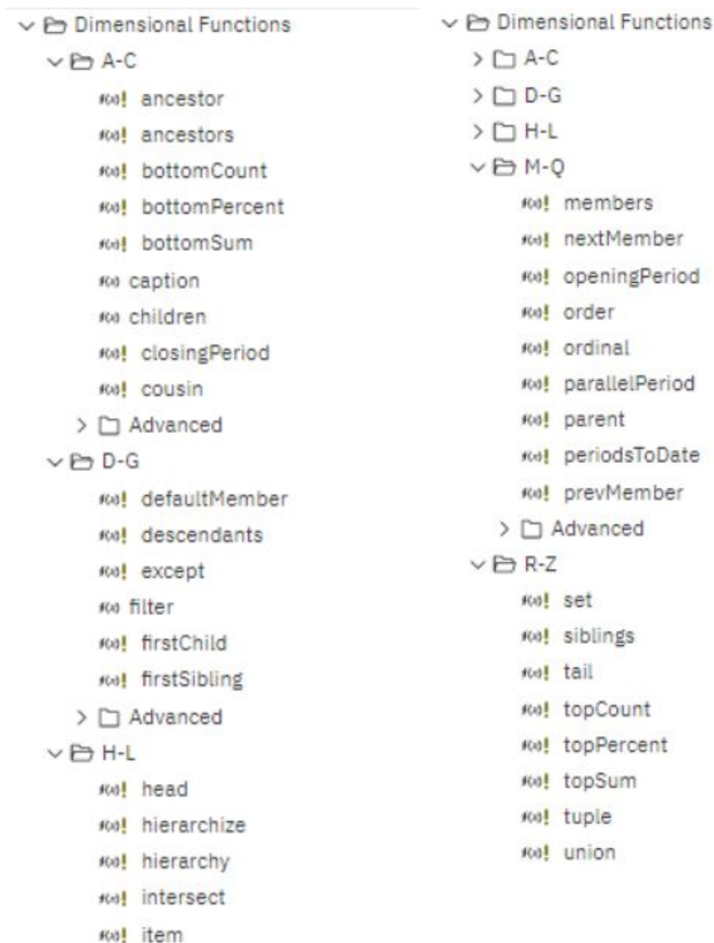
Figure 518: Insert a Query Calculation - Dimensional Functions
