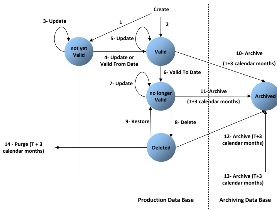
DIAGRAM 24 - LIFECYCLE OF COMMON REFERENCE DATA OBJECTS WITH LIMITED VALIDITY PERIOD
