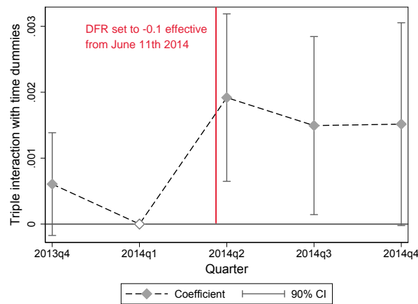
Figure 3: Evidence on the Parallel Trends Assumption
