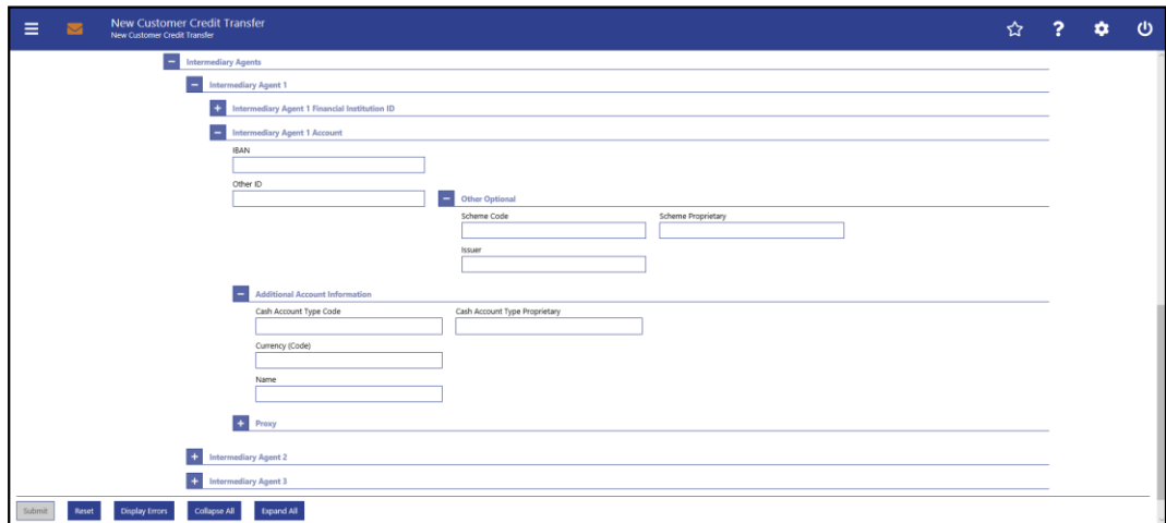
Figure 156 - CCT – New Screen – Intermediary Agent Account
