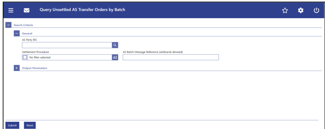
Figure 236 - Unsettled AS Transfer Orders by Batch – Query Screen
