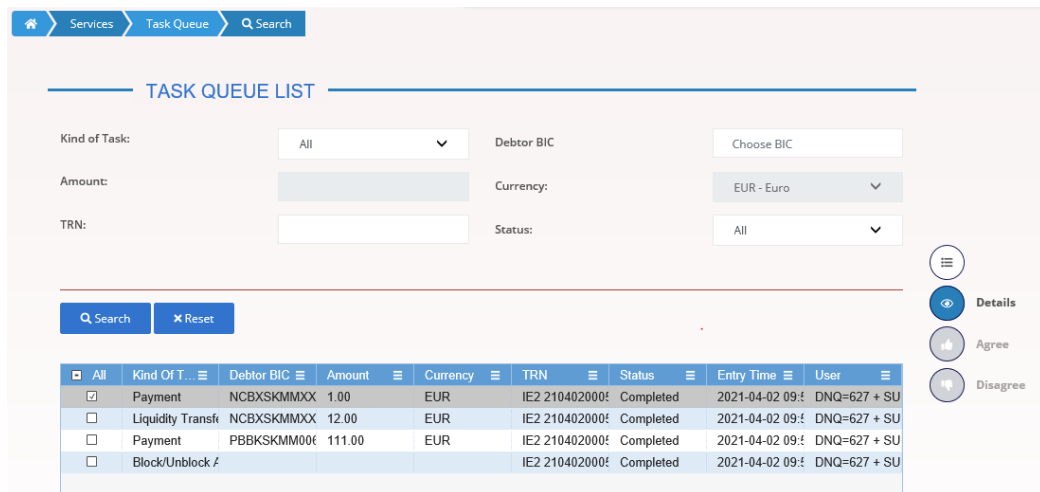
Illustration 15: Task Queue – Search/List screen
