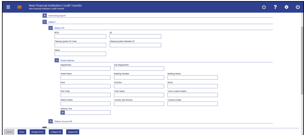
Figure 164 - FICT – New Screen – Debtor ID
