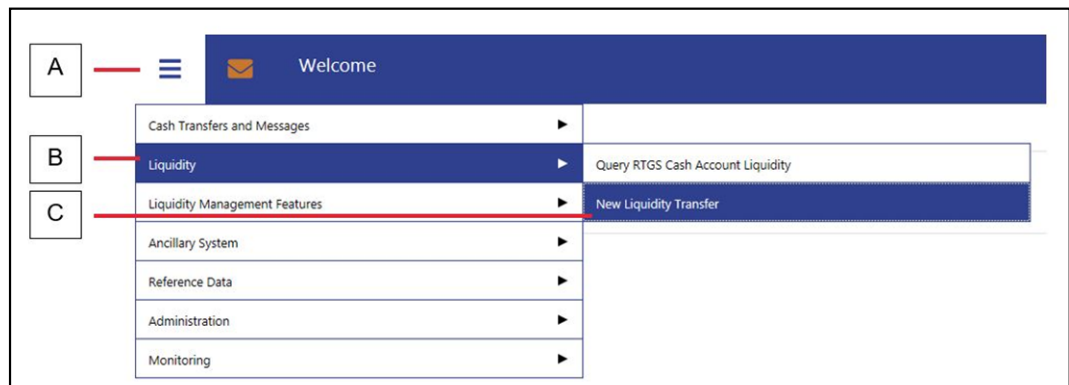
Figure 1 - RTGS Menu
