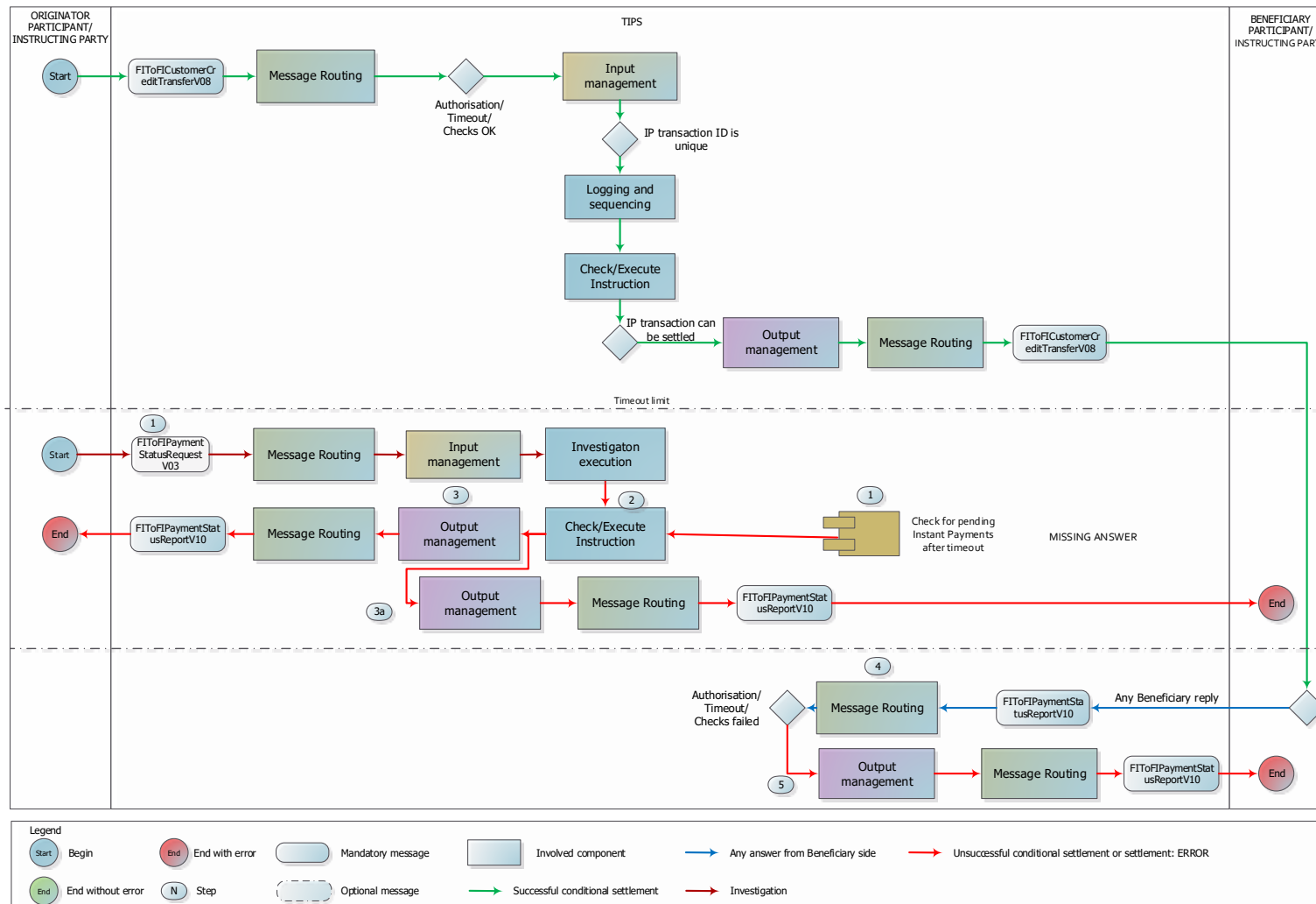
Figure 646464 – Instant Payment transaction missing/delayed Beneficiary-side answer flow (non-Euro currencies)
