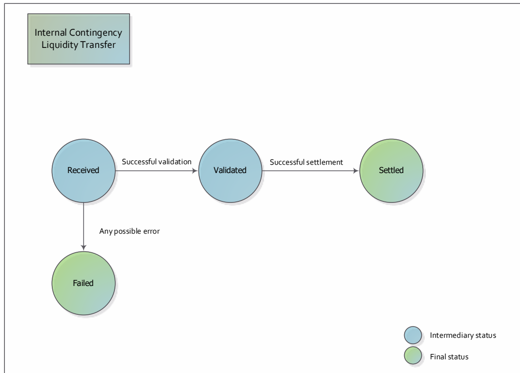
Figure 1313 – Internal Contingency Liquidity Transfer status
