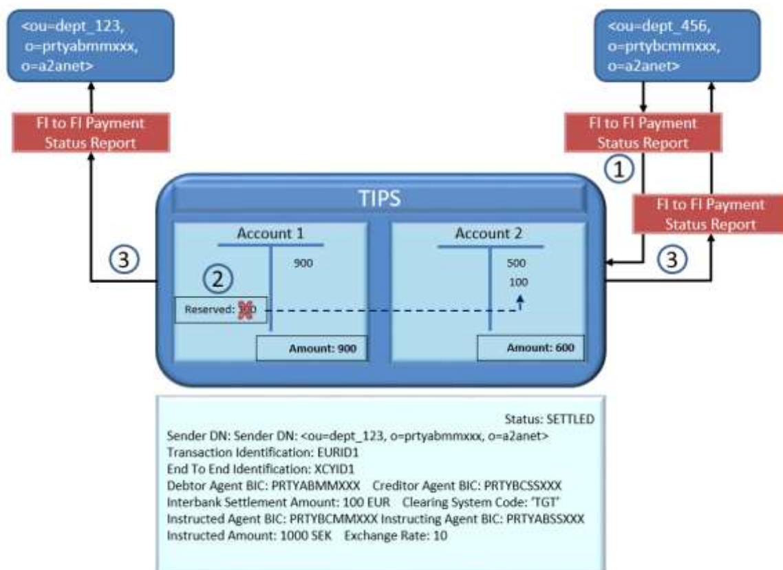
Figure 150150150 – Successful Instant Payment transaction: settlement phase in the source currency
