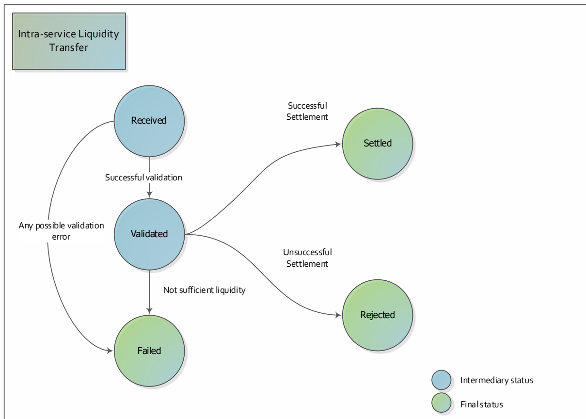
Figure 121212 – Intra-service Liquidity Transfer status diagram
