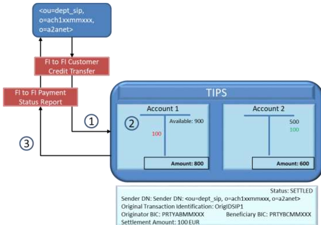
Figure 104104104 – Successful Instant Payment in Euro with SIP model: settlement phase
