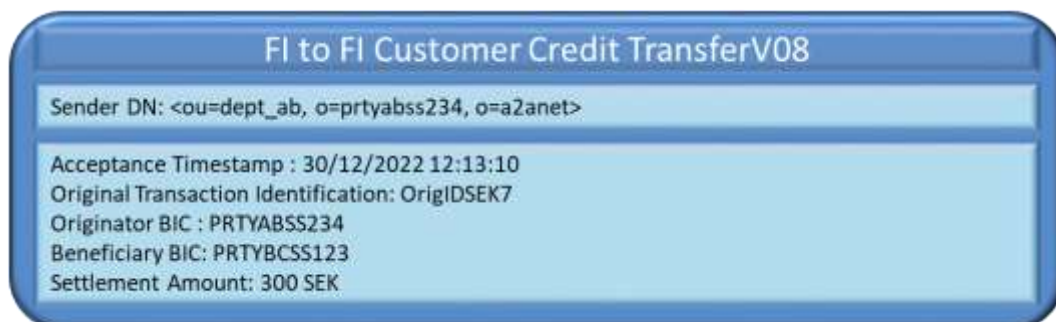
Figure 888888 – Beneficiary side timeout error: FItoFICustomerCreditTransfer
