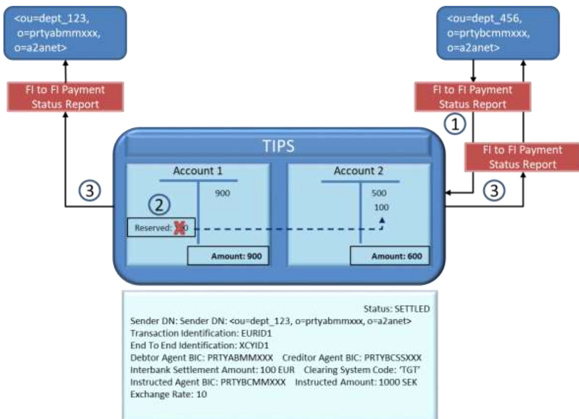
Figure 127427427 – Successful Instant Payment transaction: settlement phase
