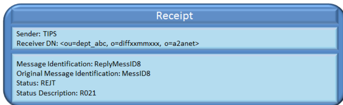
Figure 309 305285 – Unsuccessful decrease of a CMB Limit: Receipt
