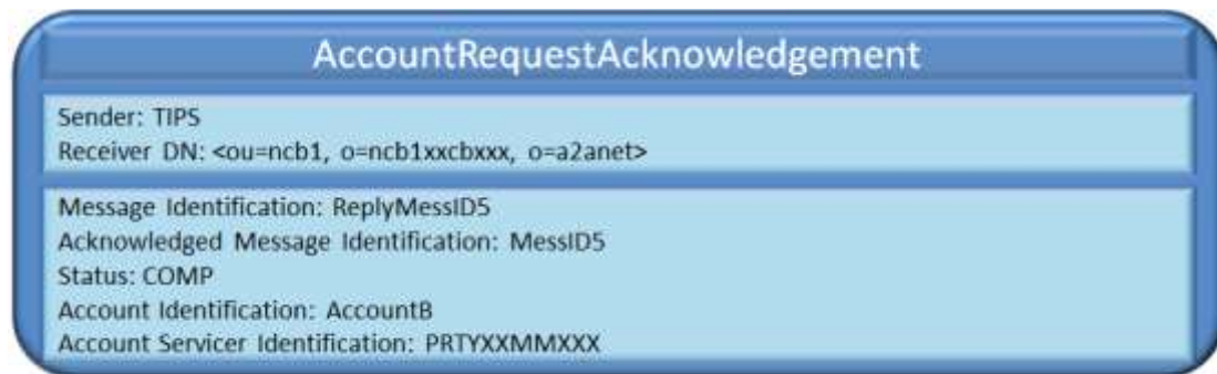
Figure 302298278 – Successful unblock of an Account: AccountRequestAcknowledgement
