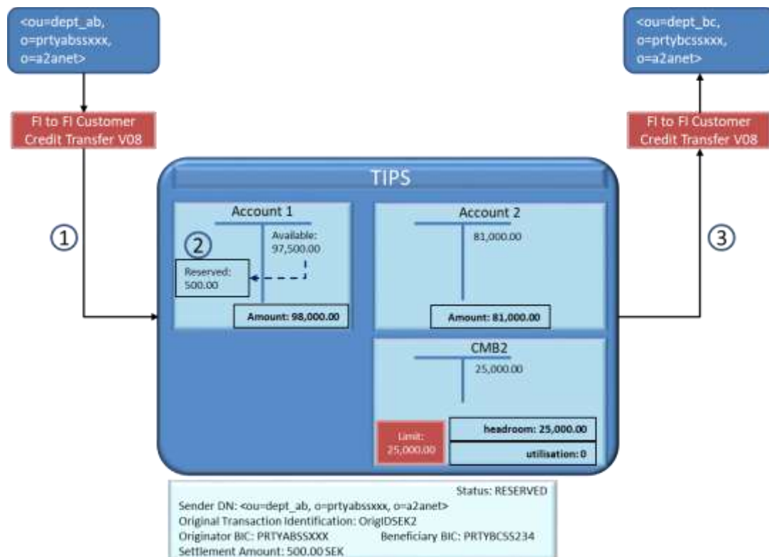
Figure 757575 – Successful Instant Payment transaction: reservation of funds
