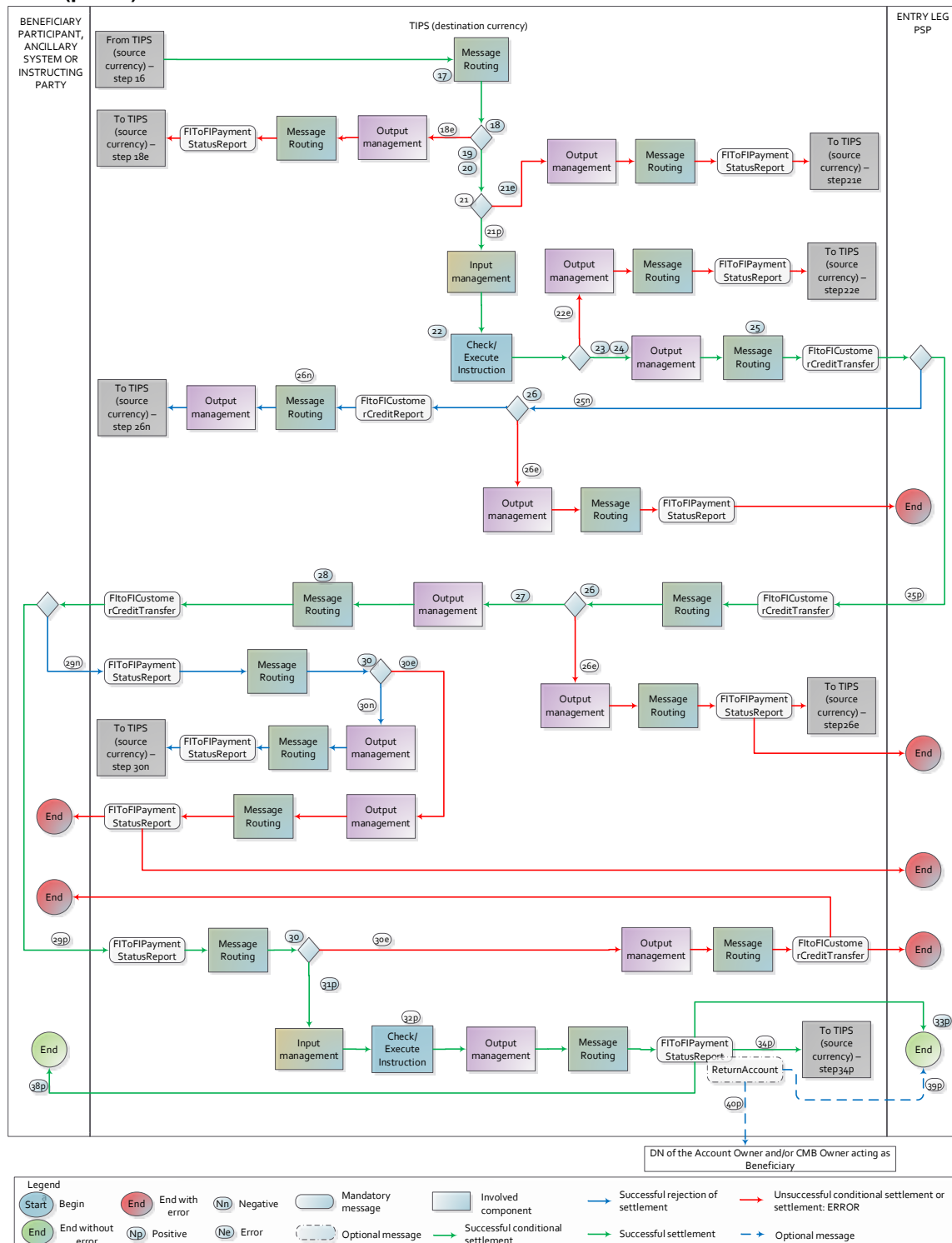
Figure 141141141 – Instant Payment transaction flow for cross-currency LKT ELKT settlement model (part II)
