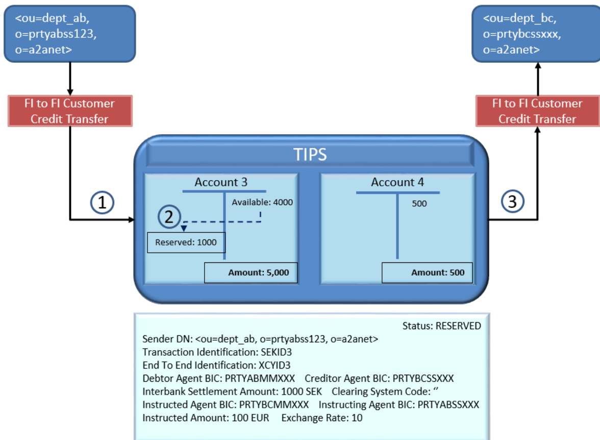
Figure 157157157 – Beneficiary side timeout: reservation of funds in the destination currency
