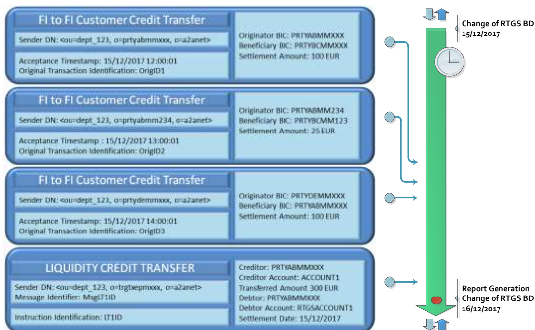
Figure 271267247 – Statement of Account Turnover example: list of transactions
