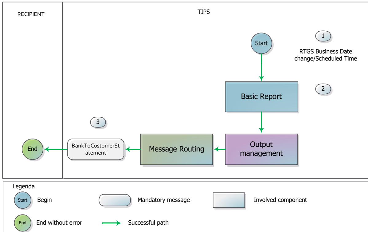
Figure 273269249 – Statement of Accounts flow
