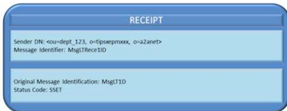
Figure 215241191 – Successful Inbound Liquidity Transfer order Receipt
