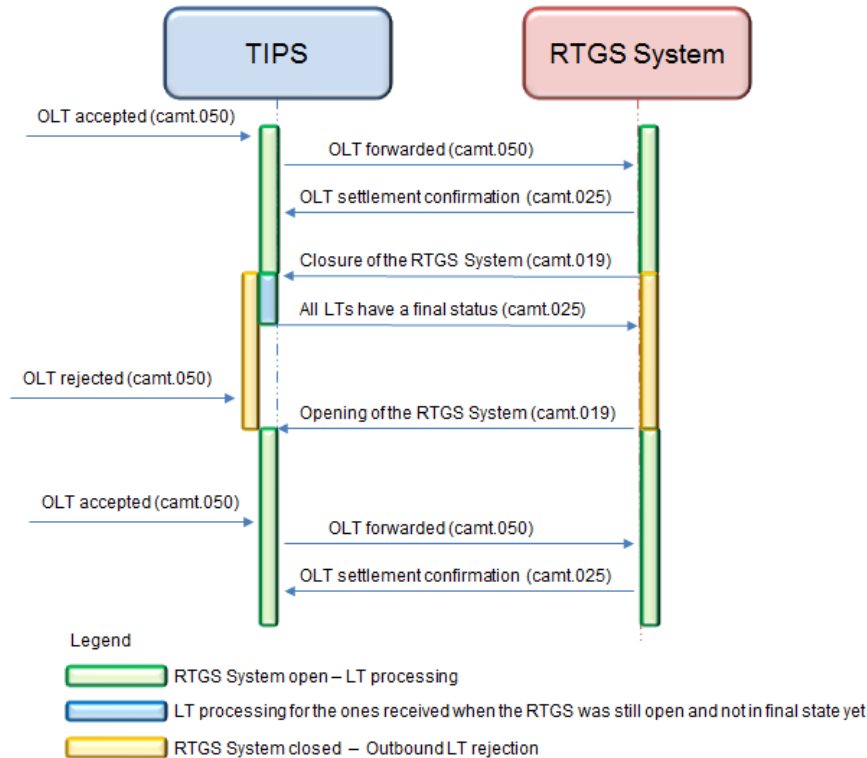
Figure 174747 – Closure and opening of the RTGS System
