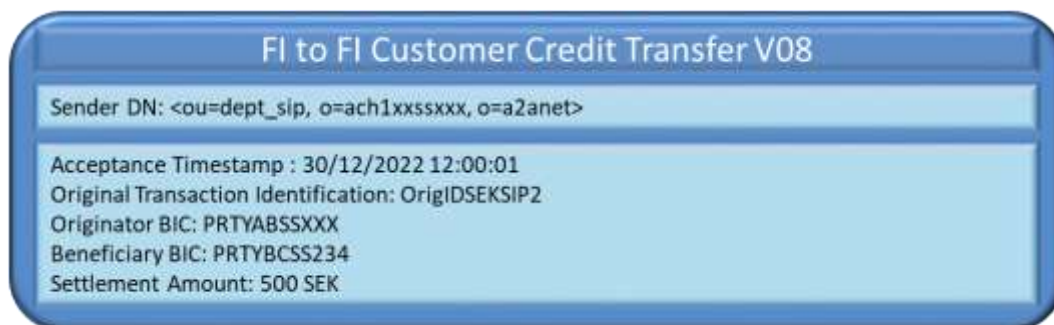
Figure 112442442 – Successful Instant Payment in non-Euro currency with SIP: FItoFICustomerCreditTransfer
