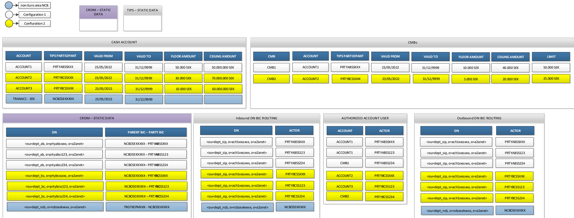
Figure 102102102 – Instant Payment transaction in a non-Euro currency - SIP settlement model - examples data constellation
