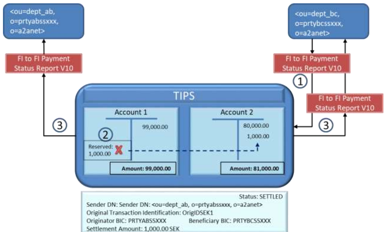
Figure 696969 – Successful Instant Payment transaction: settlement phase
