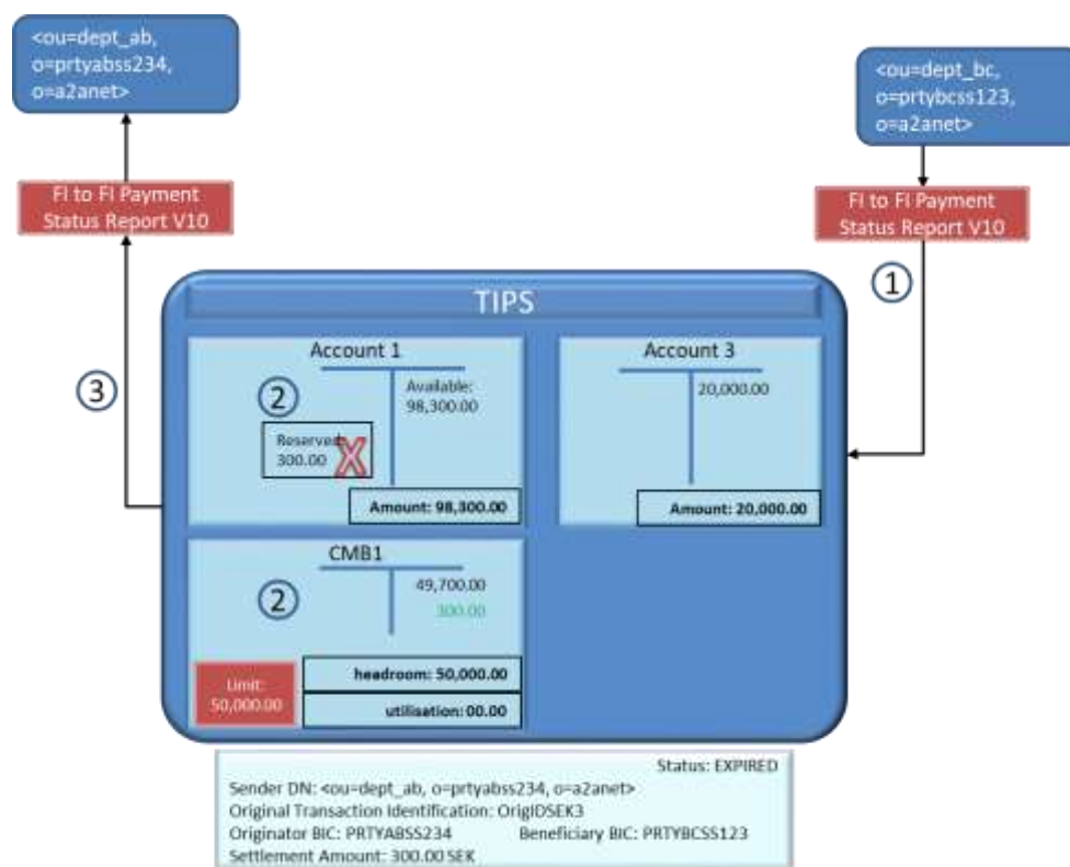
Figure 919191 – Beneficiary side timeout error: release of funds
