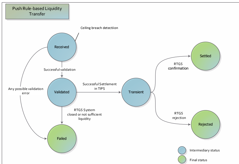
Figure 141414 – Push Rule-based Liquidity Transfer status diagram
