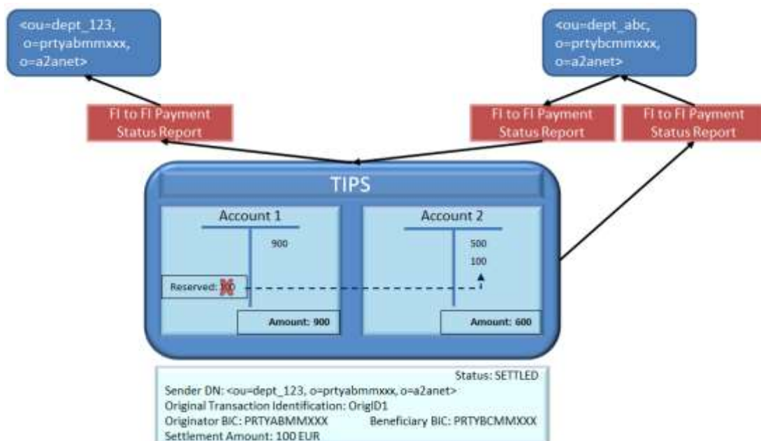
Figure 282828 – Successful Instant Payment transaction: settlement phase
