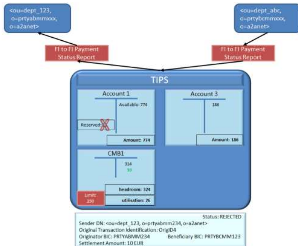
Figure 404040 – Rejected Instant Payment transaction: release of funds
