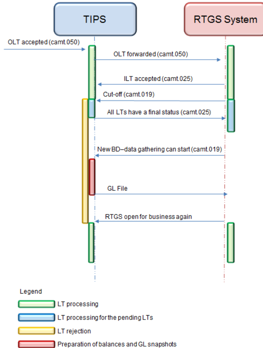
Figure 181818 – RTGS System change of business date
