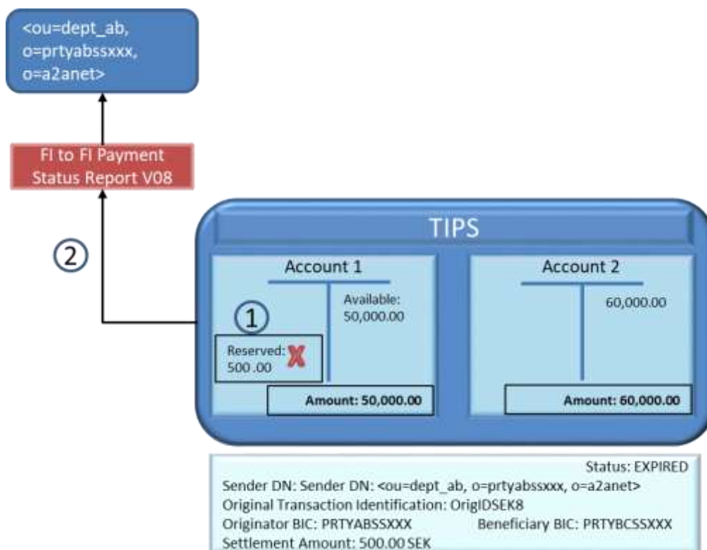
Figure 959595 – Delayed Beneficiary-side answer: release of funds
