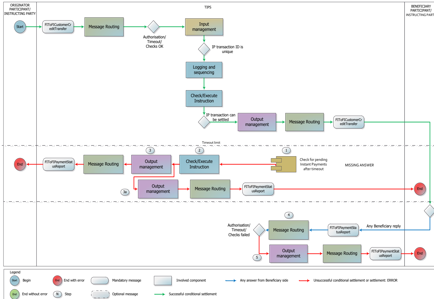
Figure 122122122 – Instant Payment transaction missing/delayed Beneficiary-side answer flow
