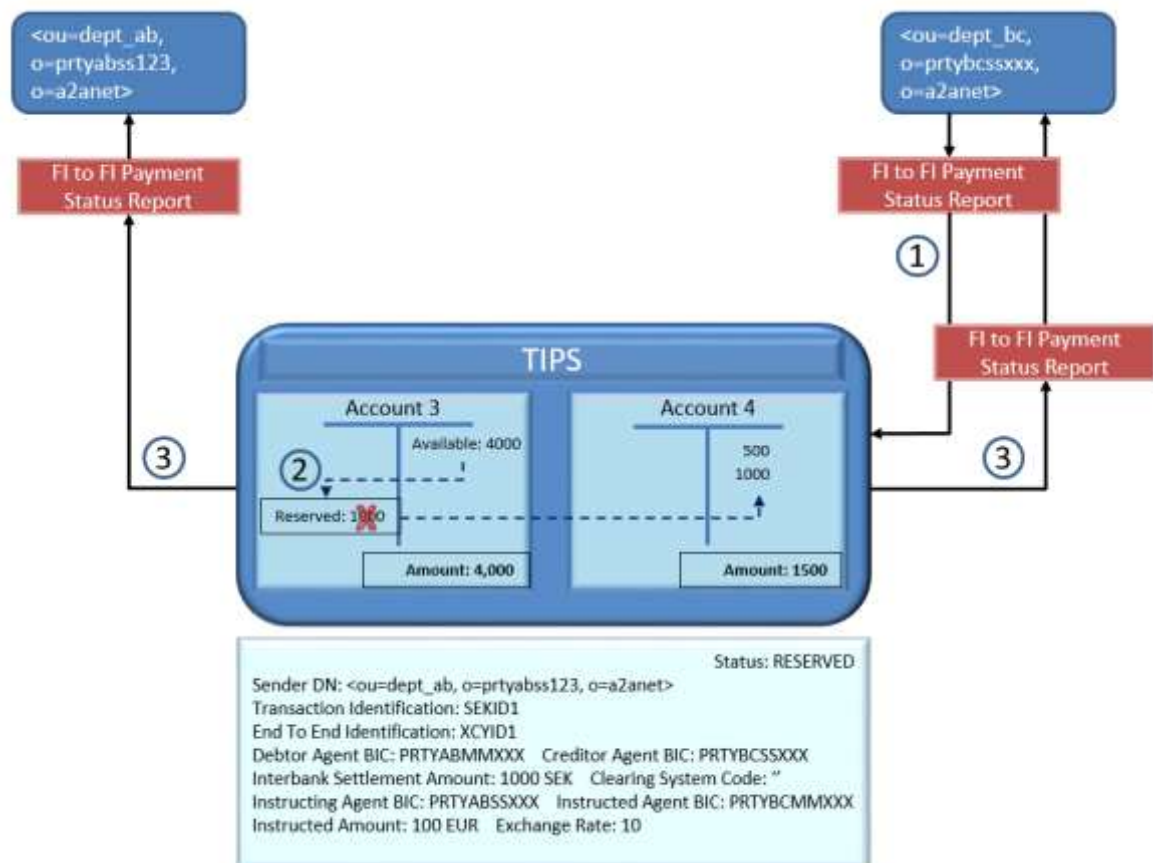
Figure 149149149 – Successful Instant Payment transaction: settlement phase in the destination currency
