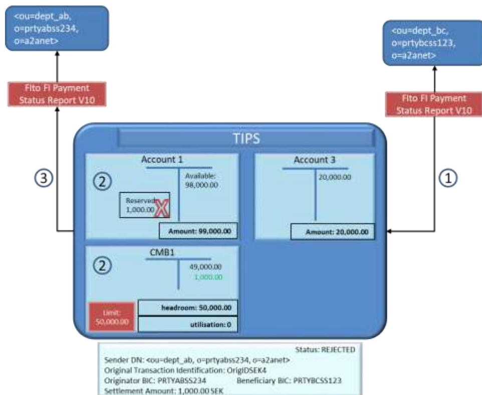
Figure 818184 – Rejected Instant Payment transaction: release of funds
