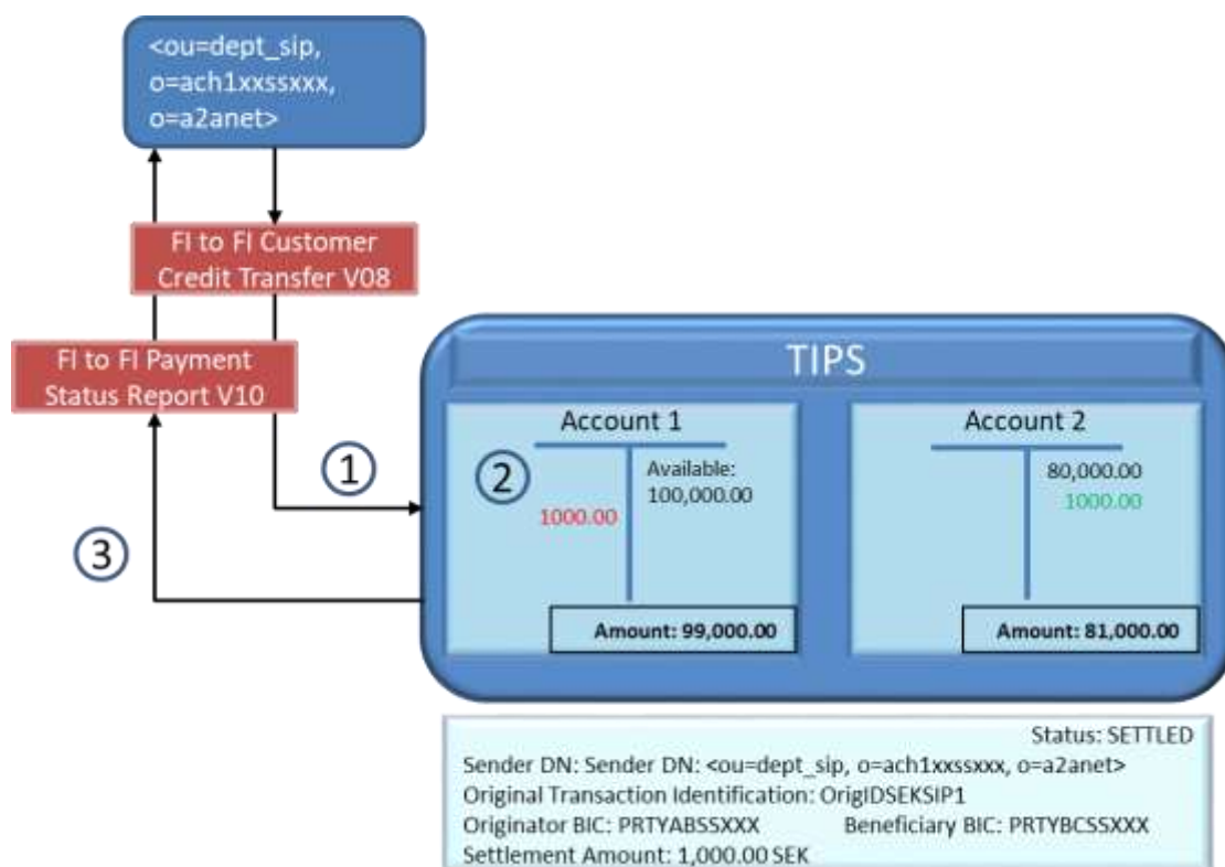
Figure 110110110 – Successful Instant Payment in non-Euro currency with SIP: settlement phase
