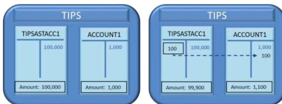
Figure 182180178 – Recall successful scenario: positive response – Settlement Process
