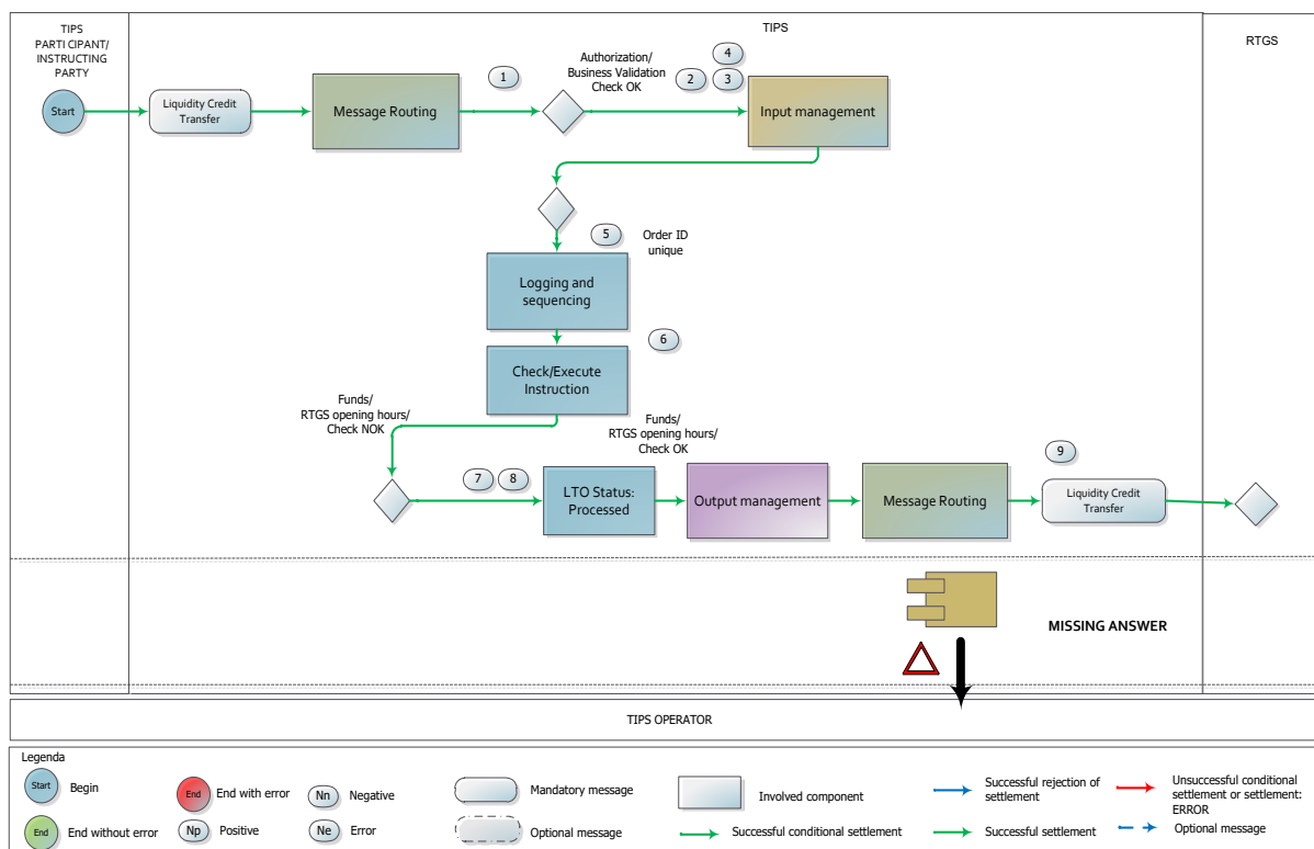
Figure 236232212 – Outbound Liquidity Transfer: Missing RTGS System answer flow
