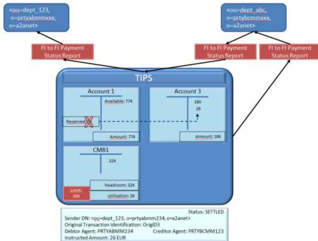
Figure 323232 – Successful Instant Payment transaction: settlement phase
