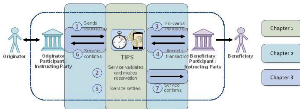
Figure 144 – Scope of UDFS
