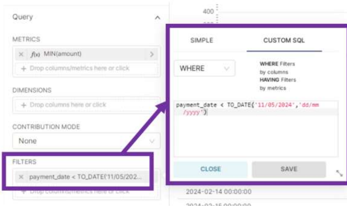
Figure 313309289 – Example of custom SQL filter on payment_date
