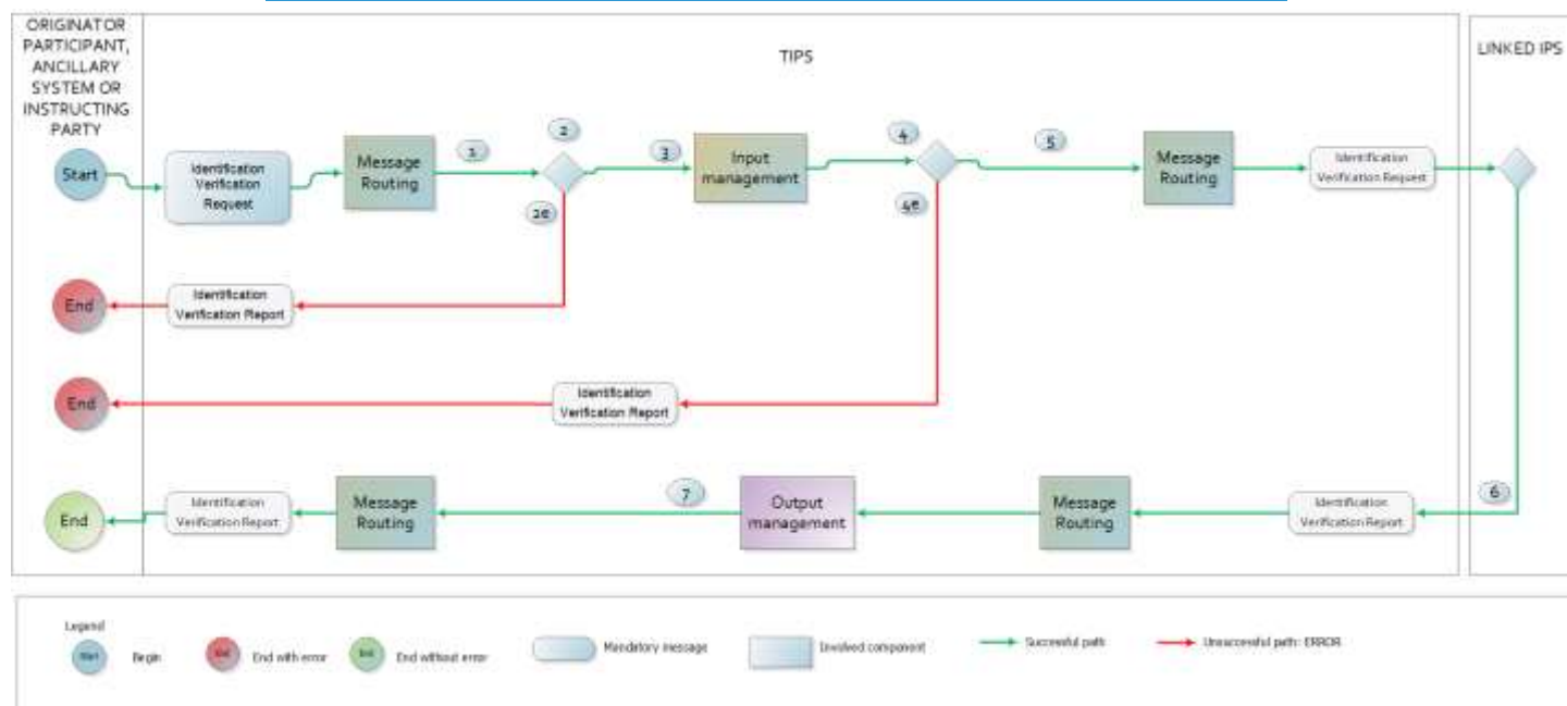
Figure 162 - TIPS outgoing Instant Payment validation flow for interlinking
