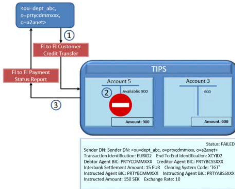
Figure 152152152 – Blocked account error: transaction failed
