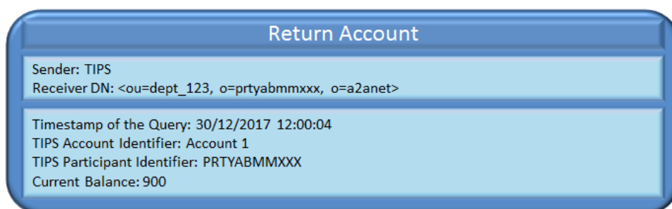
Figure 250246226 – Floor notification ReturnAccount
