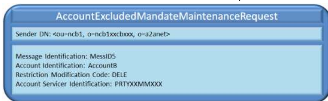
Figure 300296276 – Successful unblock of an Account: AccountExcludedMandateMaintenanceRequest
