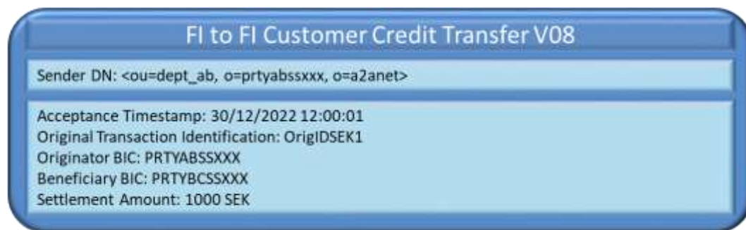
Figure 666666 – Successful Instant Payment transaction: FItoFICustomerCreditTransfer
