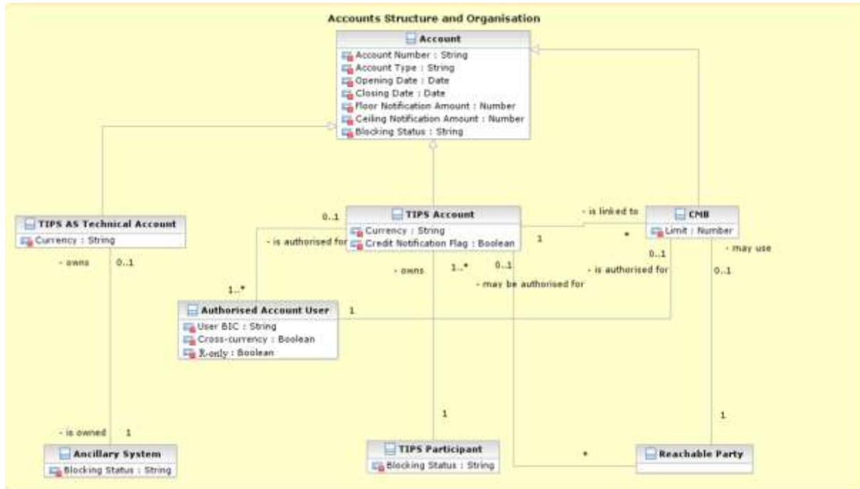
Figure 444 – Account structure and organisation
