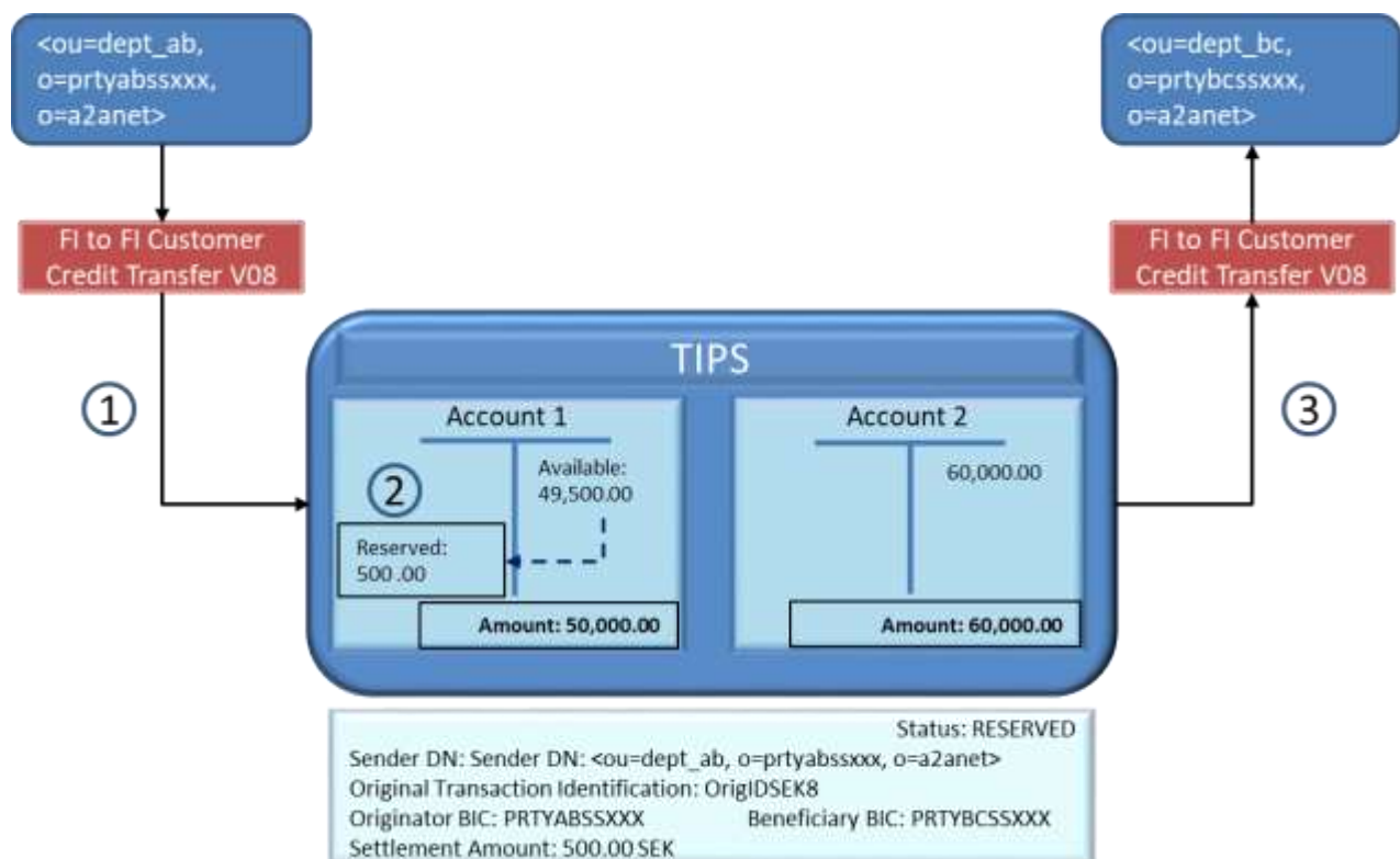
Figure 949494 – Delayed Beneficiary-side answer: reservation of funds
