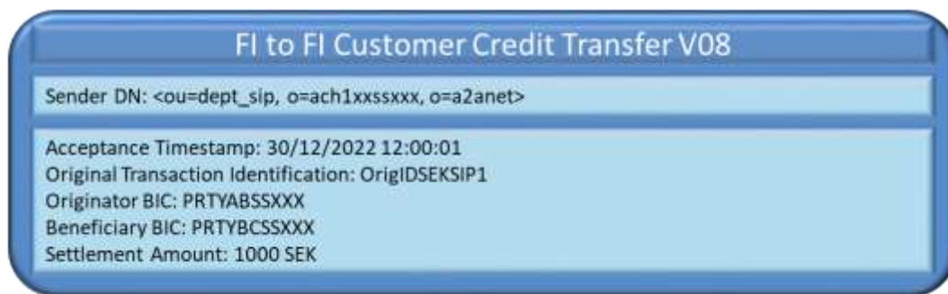
Figure 109 109 109 – Successful Instant Payment in non-Euro currency with SIP: FIToFICustomerCreditTransfer
