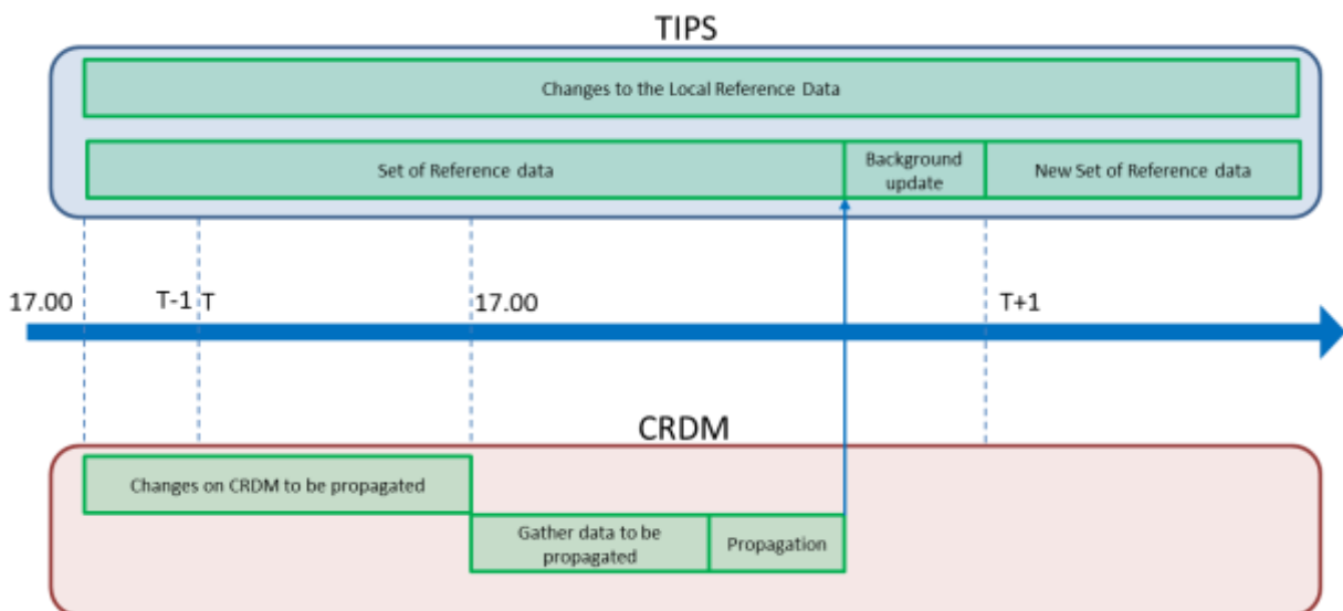
Figure 202020 – Interaction between CRDM and TIPS 27
