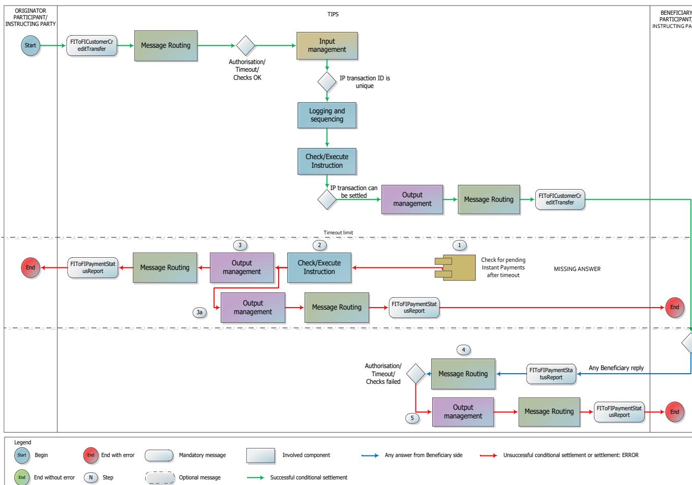
Figure 232323 – Instant Payment transaction missing/delayed Beneficiary-side answer flow
