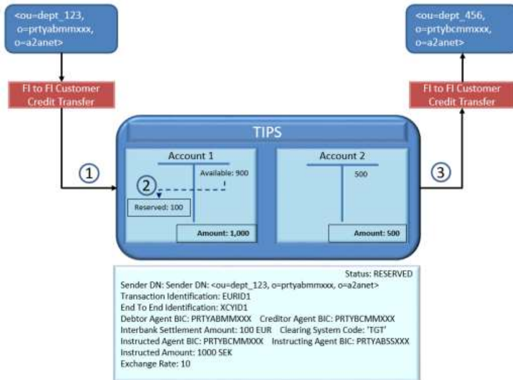
Figure 144144144 – Successful Instant Payment transaction: Reservation of EUR amount
