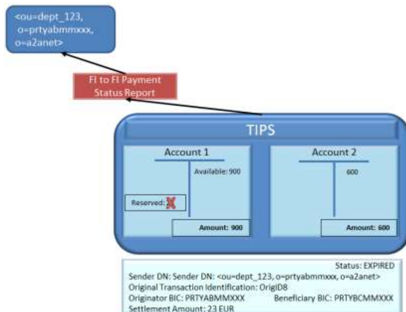
Figure 585858 – Delayed Beneficiary-side answer: release of funds
