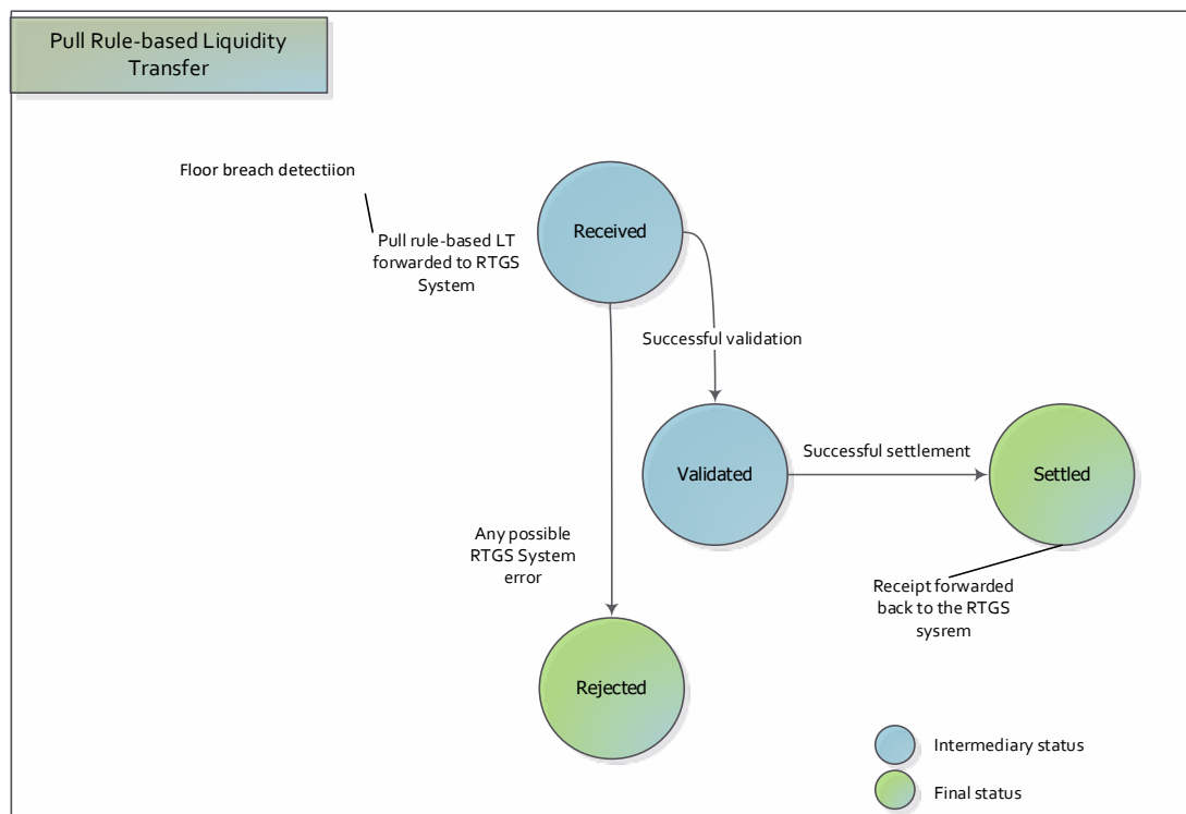
Figure 151515 - Pull rule-based Liquidity Transfer status diagram
