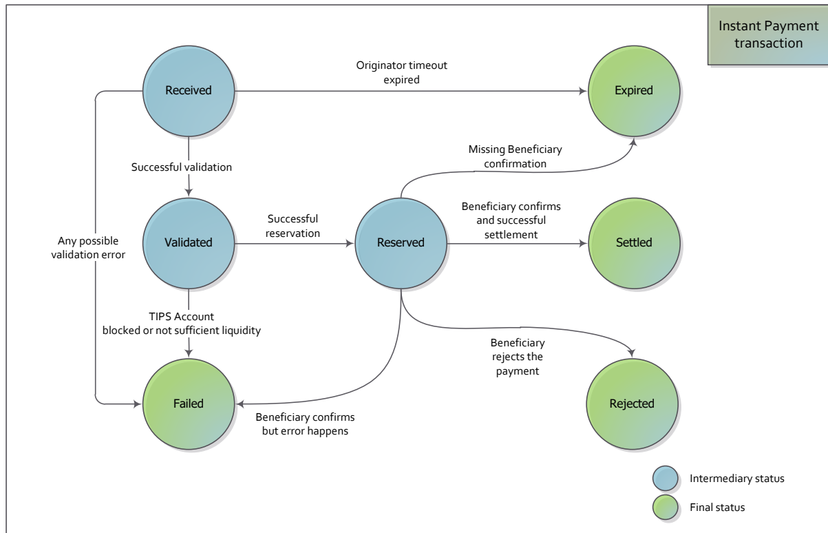
Figure 666 – Instant Payment Transaction status transition diagram
