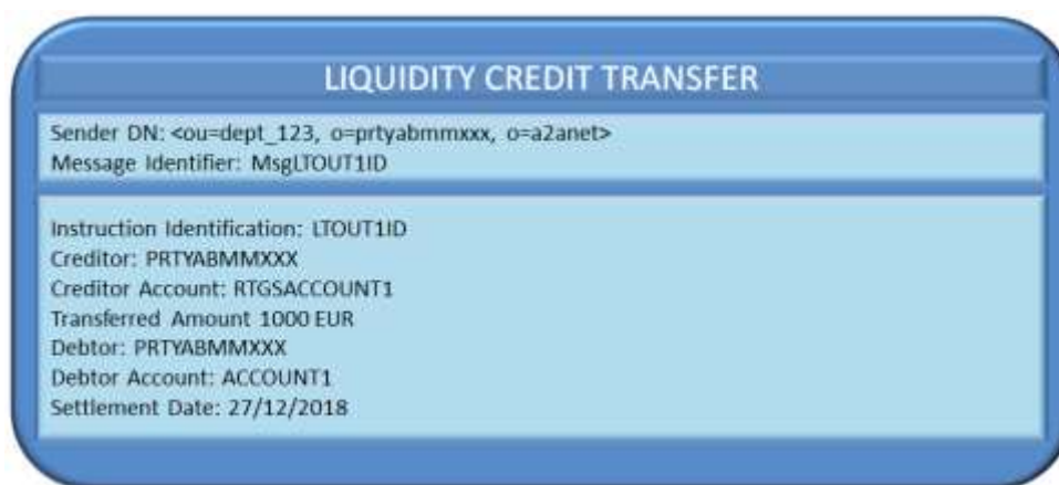
Figure 230226206 – Outbound Liquidity Transfer order: incoming message
