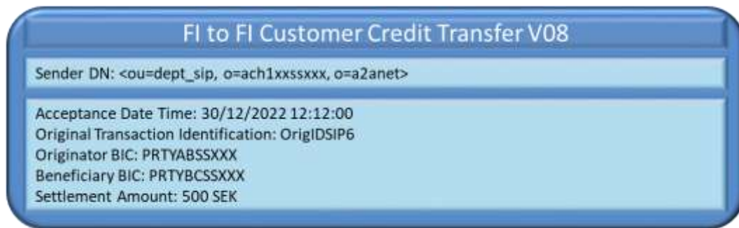
Figure 118118118 – Blocked account error: FItoFICustomerCreditTransfer
