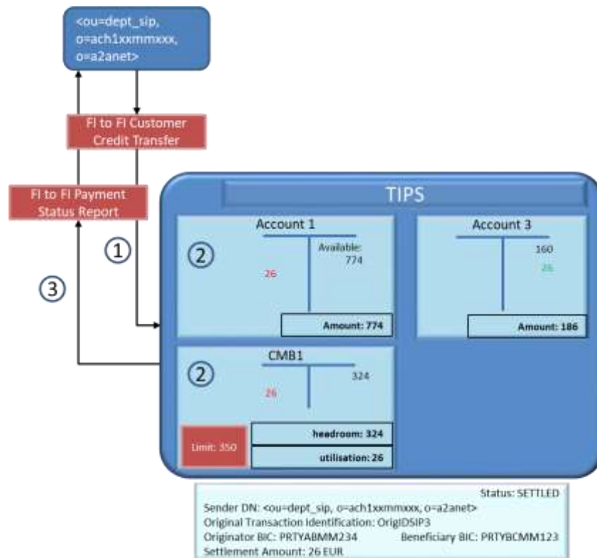
Figure 107107107 – Successful Instant Payment in non-Euro currency with SIP: settlement phase
