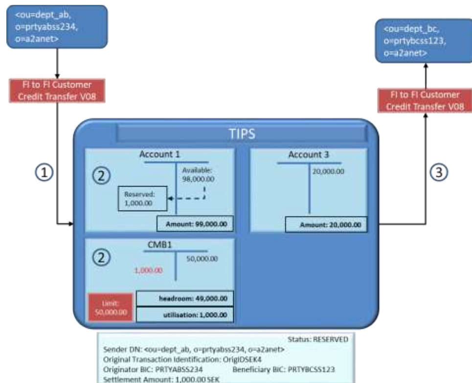
Figure 797979 – Rejected Instant Payment transaction: reservation of funds
