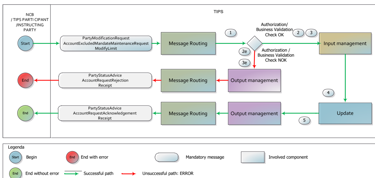
Figure 284280260 – Reference Data Messages flow
