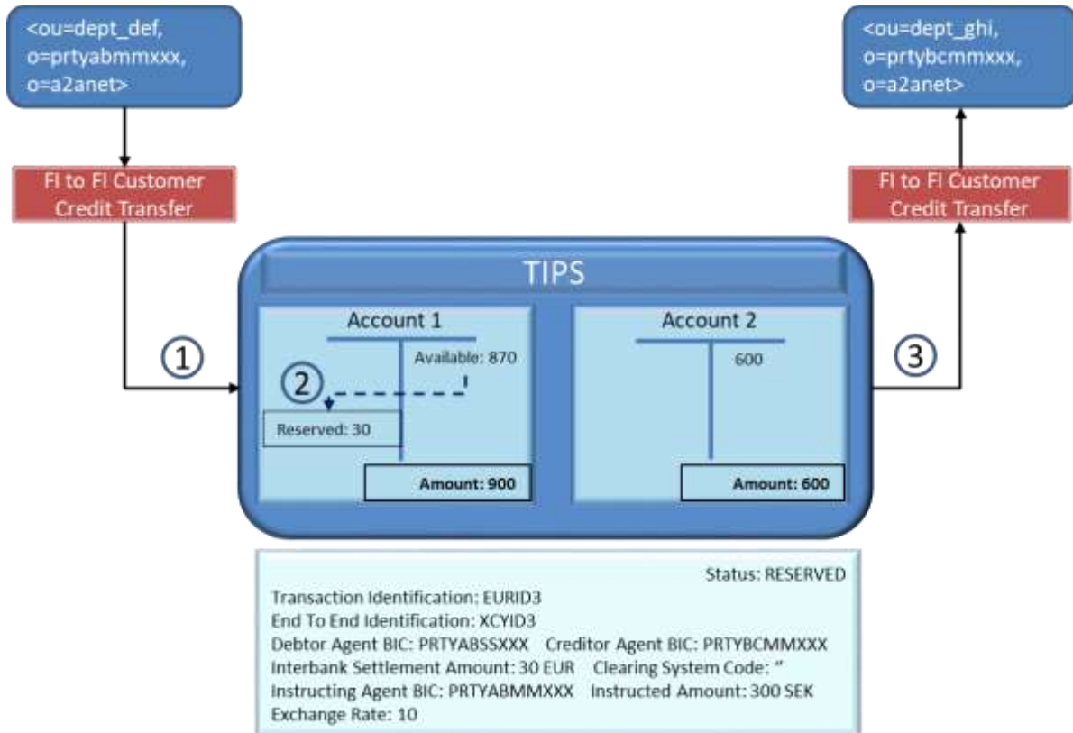
Figure 136136136 – Beneficiary side timeout error: reservation of funds
