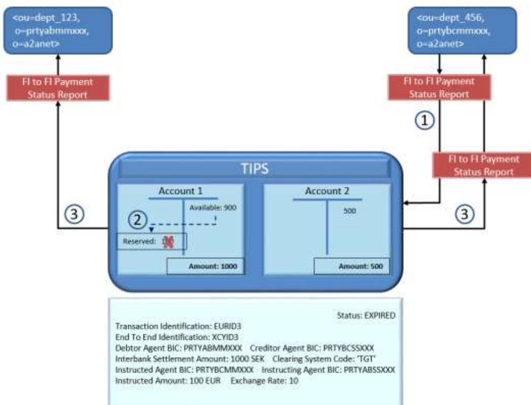
Figure 161161161 – Beneficiary side timeout: release of funds in the source currency
