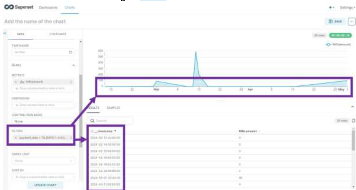
Figure 312308288 – Additional filters
