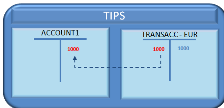
Figure 234230240 – Outbound Liquidity Transfer order: reverse settlement
