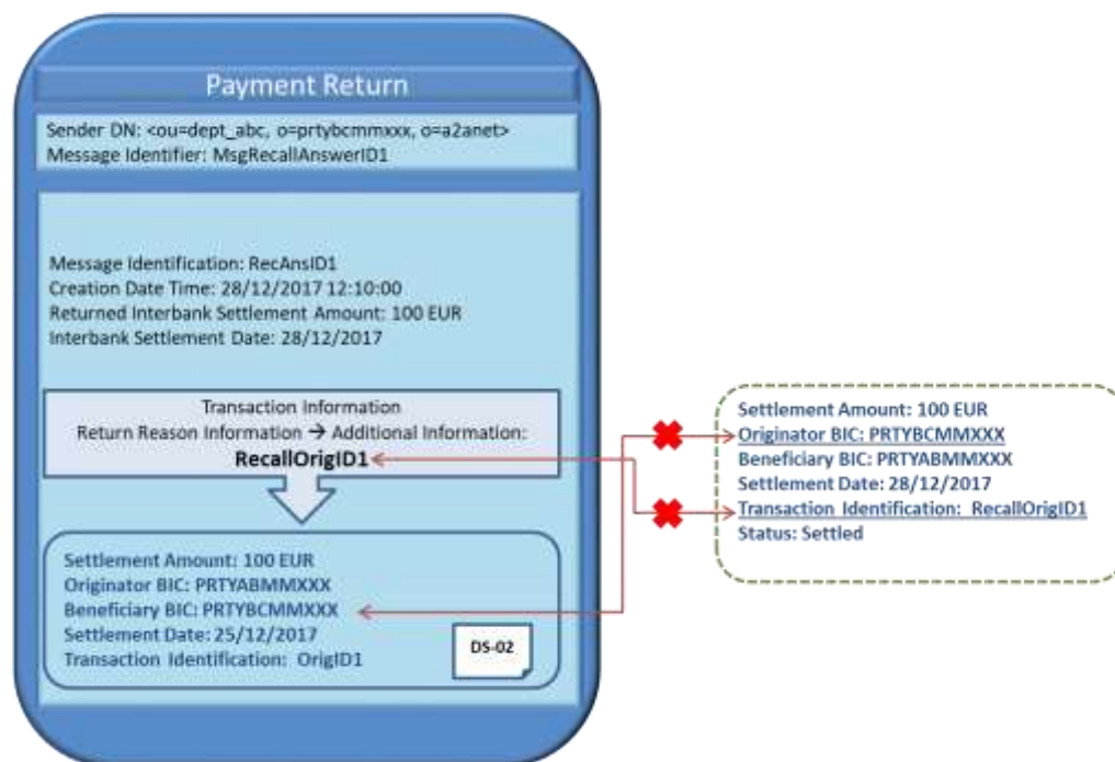
Figure 176174172 – Recall unsuccessful scenario: Duplicate check failed – Duplicate submission
