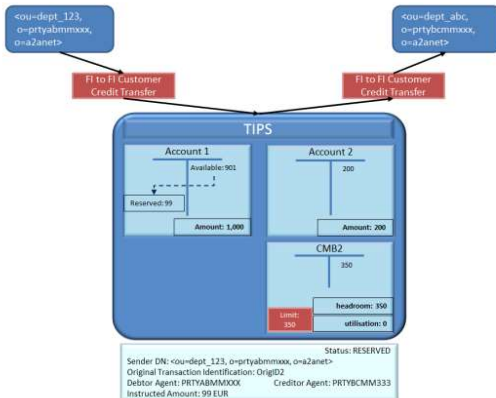
Figure 343434 – Successful Instant Payment transaction reservation of funds
