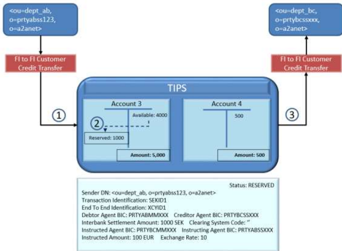
Figure 147147147 – Successful Instant Payment transaction: reservation of SEK amount
