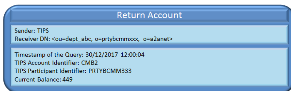
Figure 252 248 228 – Ceiling notification ReturnAccount
