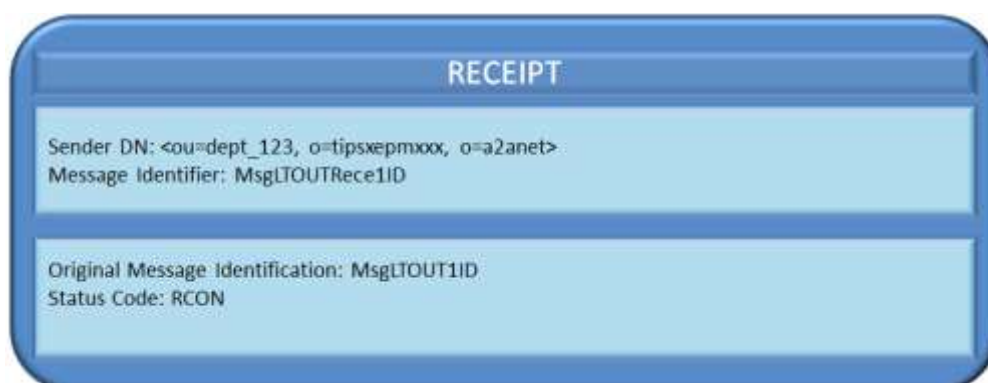
Figure 226222202 – Successful Outbound Liquidity Transfer order Receipt sent by TIPS
