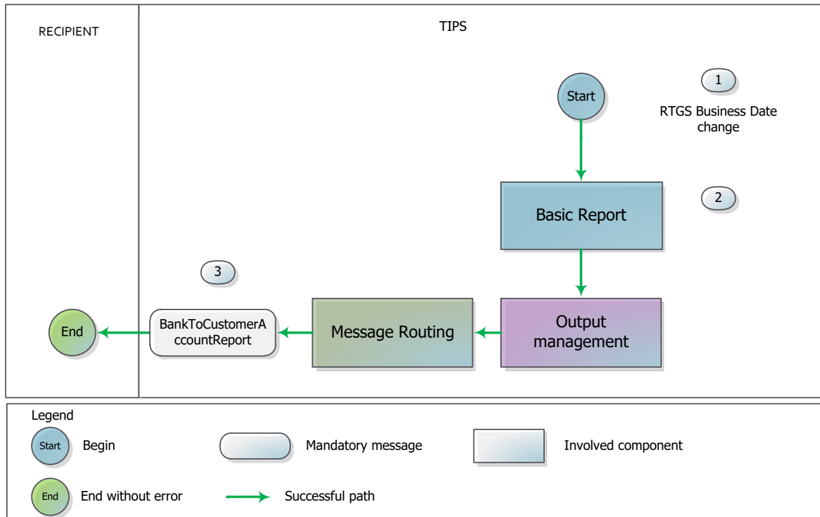
Figure 268264244 – Statement of Account Turnover flow
