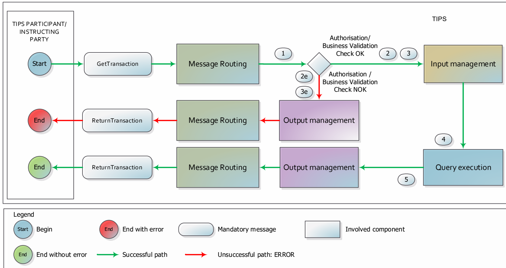
Figure 254250230 – Payment transaction status query flow
