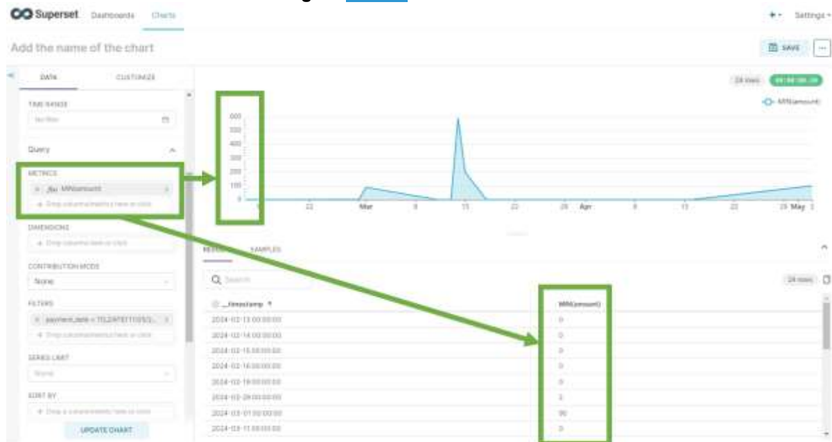
Figure 311307287 – Metrics field
