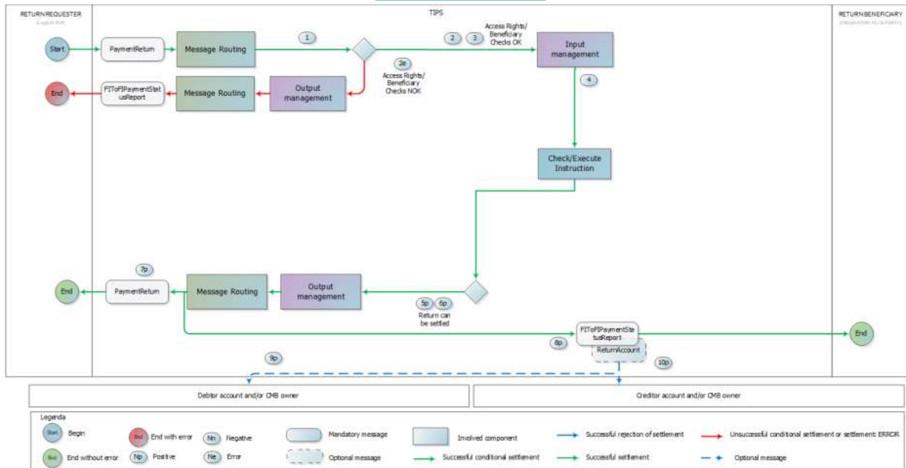
Figure 193191 - Return flow
