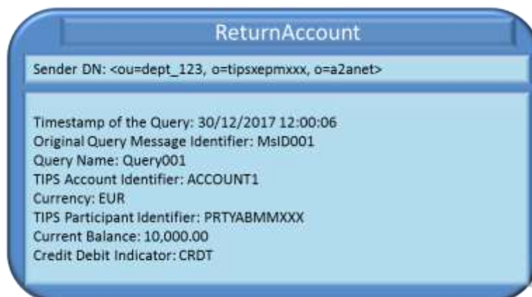
Figure 257253233 – Successful ReturnAccount
