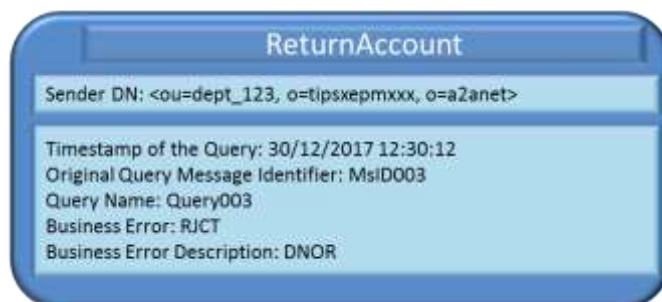
Figure 262 258 238 – Unsuccessful ReturnAccount
