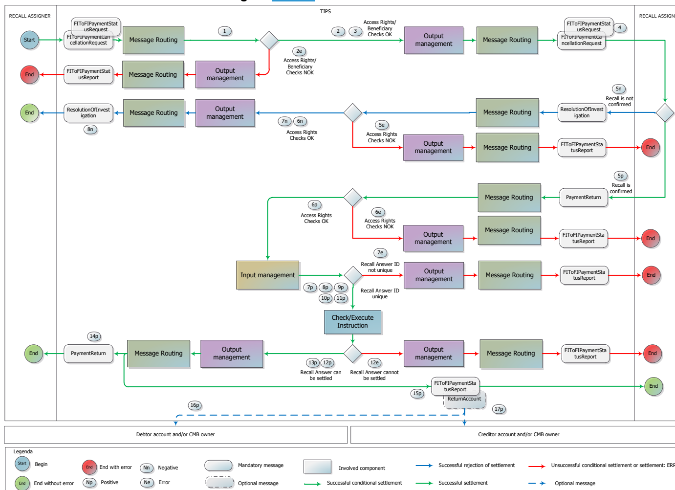
Figure 166164162 – Recall flow
