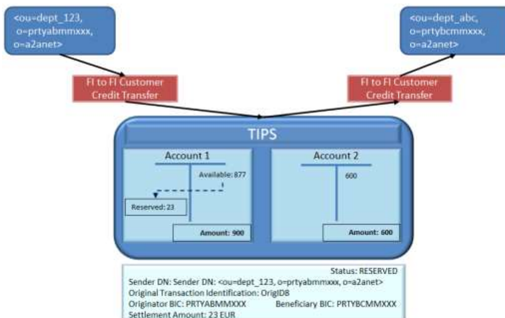
Figure 575757 – Delayed Beneficiary-side answer: reservation of funds
