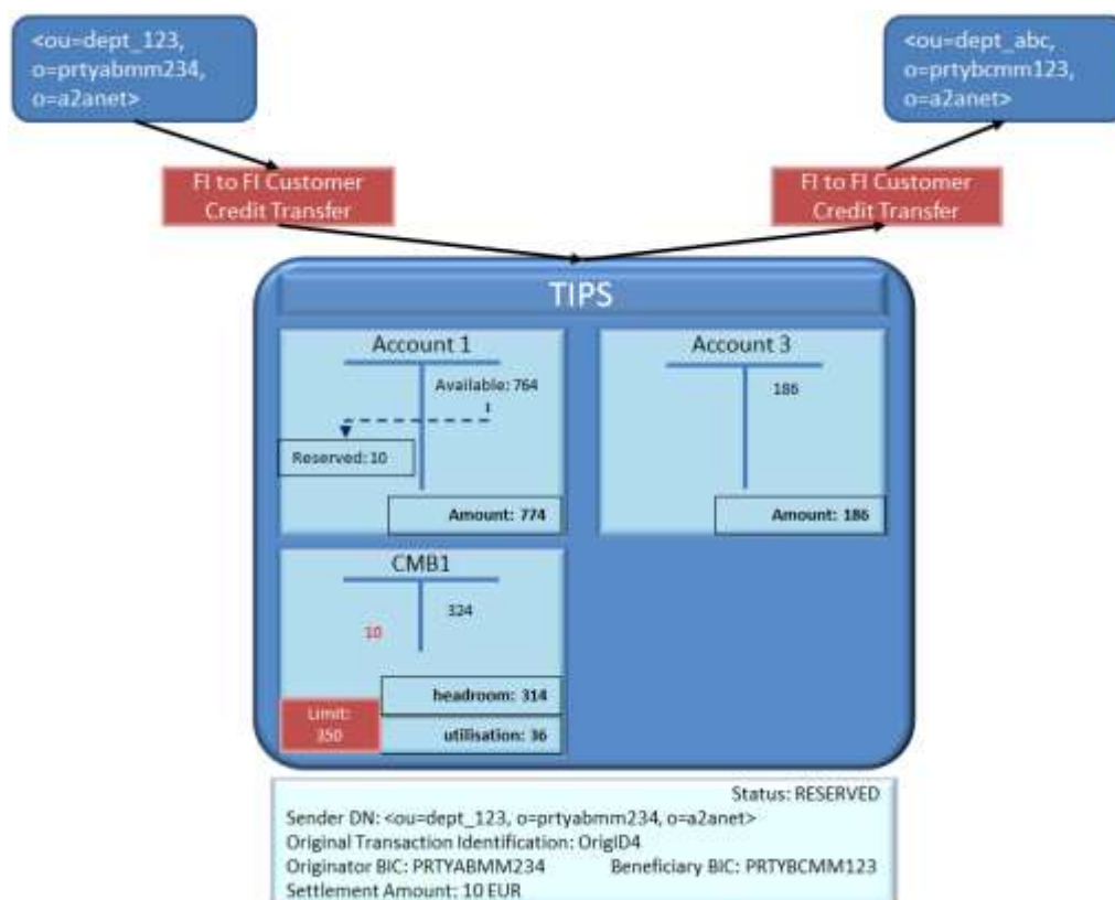
Figure 383838 – Rejected Instant Payment transaction: reservation of funds
