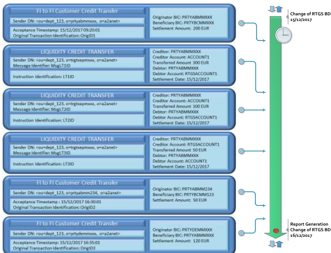
Figure 277273253 – Statement of Accounts example: list of transactions (full mode)
