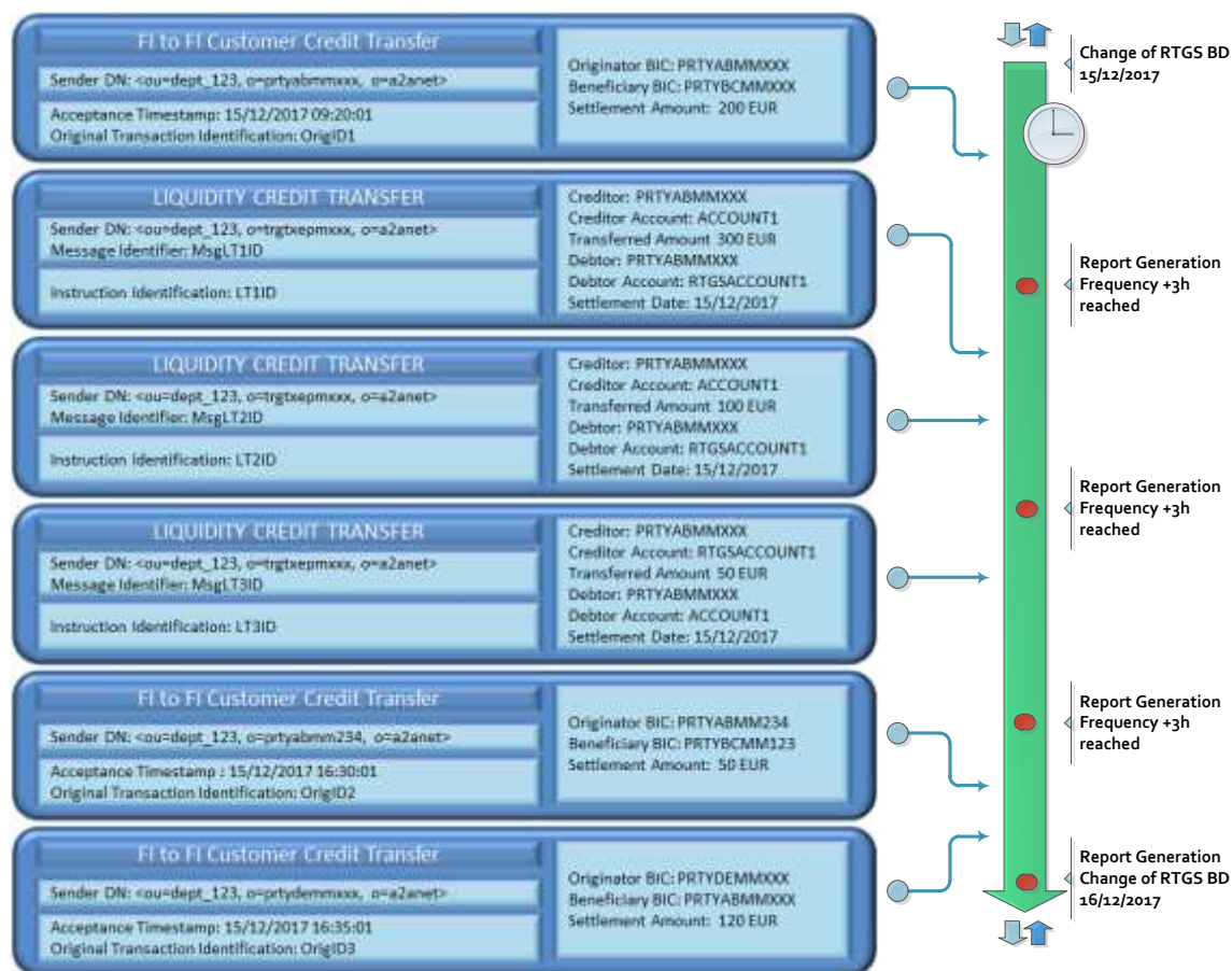
Figure 279275255 – Statement of Accounts example: list of transaction (delta mode)
