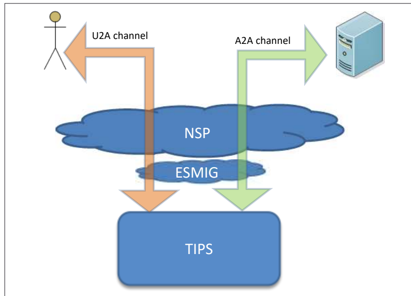
Figure 222 – TIPS Connectivity
