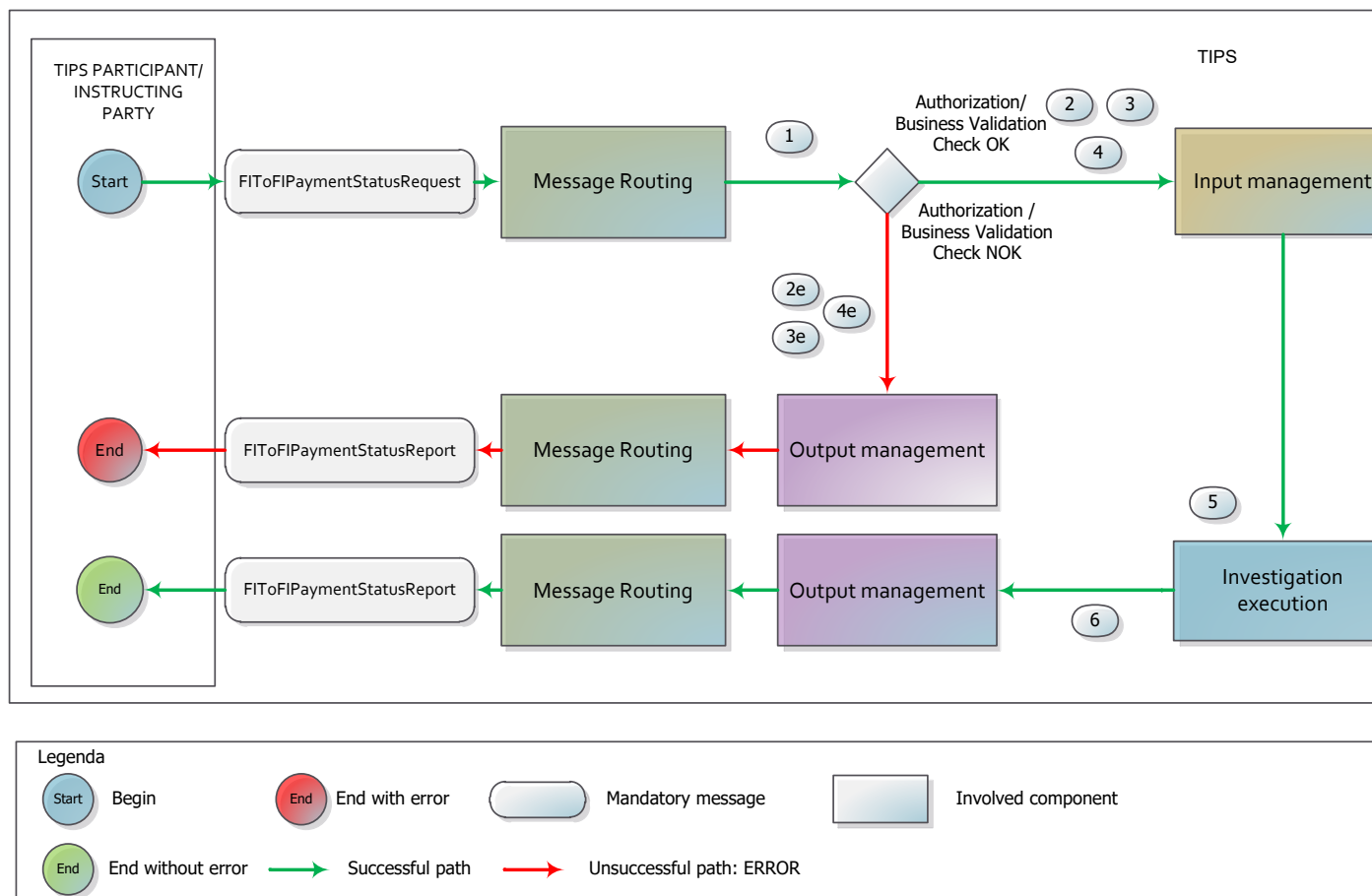
Figure 197495179 – Investigation Flow
