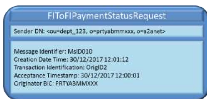
Figure 201197184 – Successful FIToFIPaymentStatusRequest
