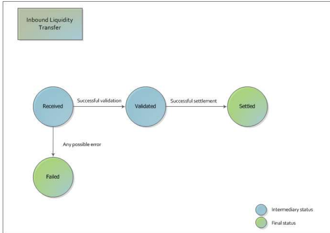
Figure 101010 – Inbound Liquidity Transfer status diagram
