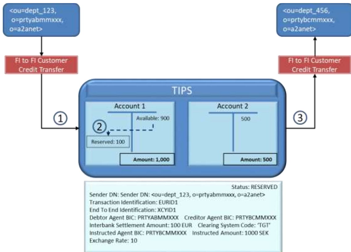
Figure 125125125 – Successful Instant Payment transaction: reservation of funds
