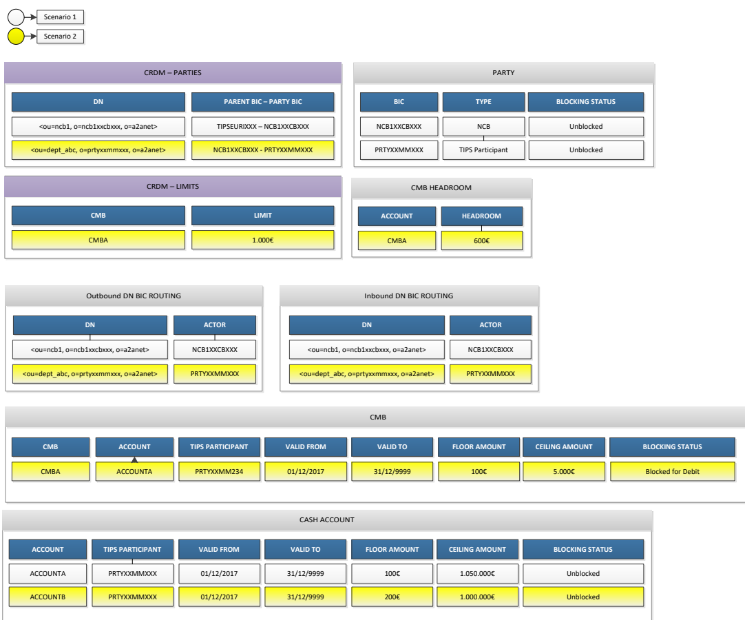
Figure 285281261 – Reference Data Management examples: data constellation
