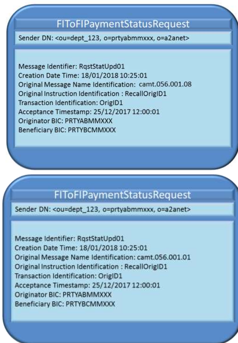
Figure 178176174 – Successful request for Status Update on a Recall
