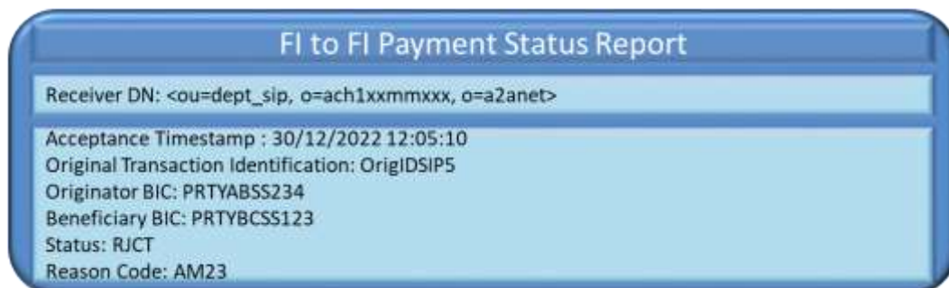
Figure 117447447 – Headroom error: FItoFIPaymentStatusReport
