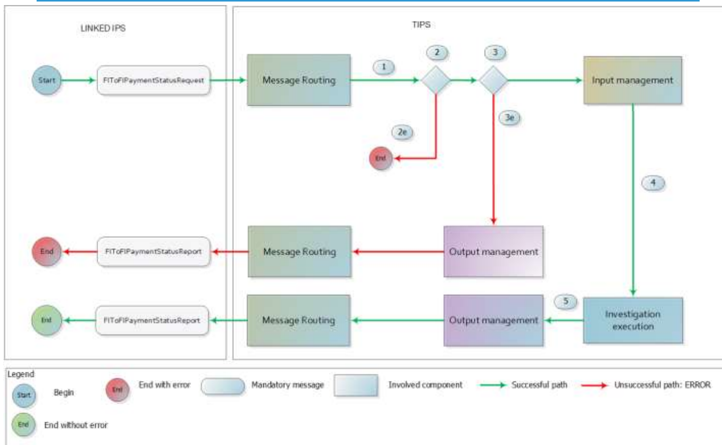
Figure 198 - Investigation flow of cross currency Instant Payment transactions from Linked IPS to TIPS
