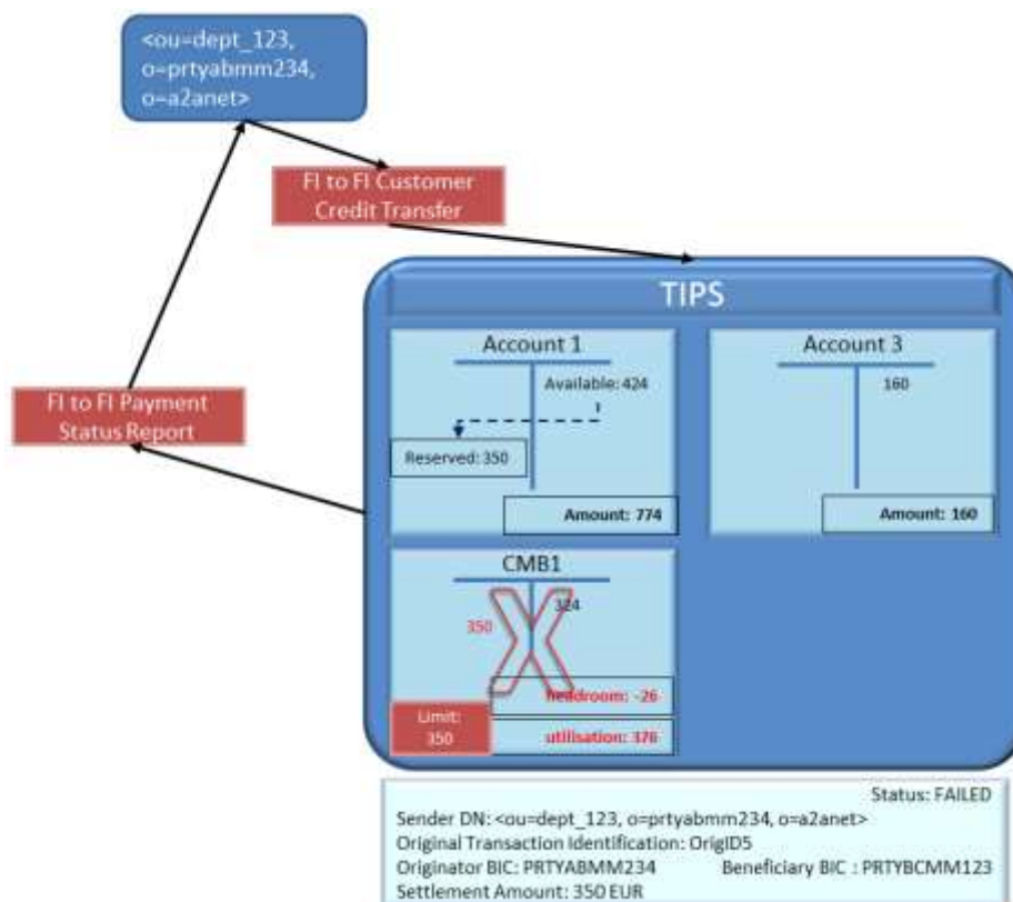
Figure 464646 – Headroom error: transaction failed
