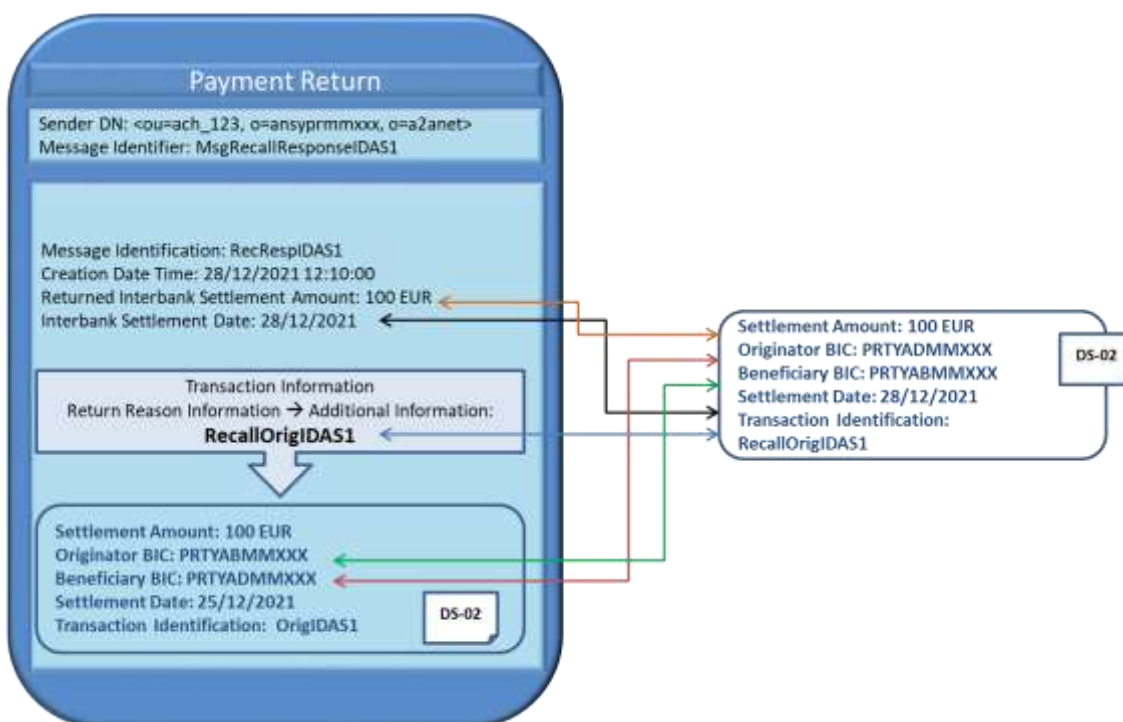
Figure 181179177 – Recall successful scenario: positive response – Recall Dataset
