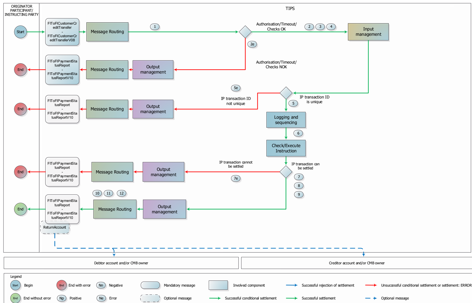
Figure 100100100 – Instant Payment transaction flow for SIP settlement model
