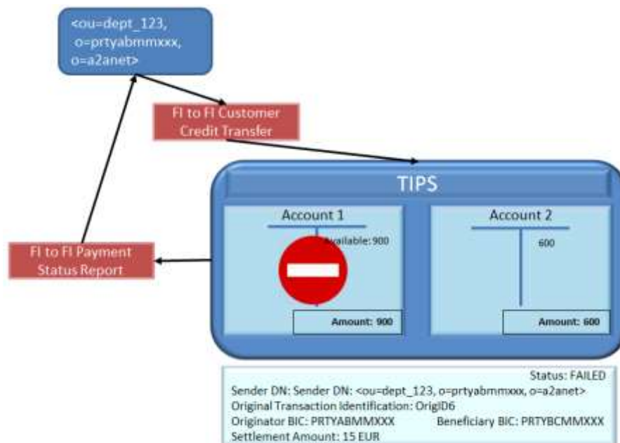
Figure 494949 – Blocked account error: transaction failed
