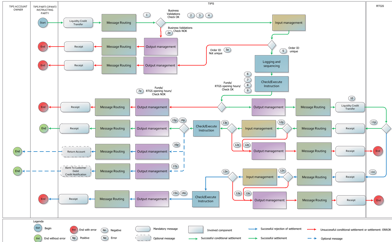
Figure 220246196 – Outbound Liquidity Transfer Order flow
