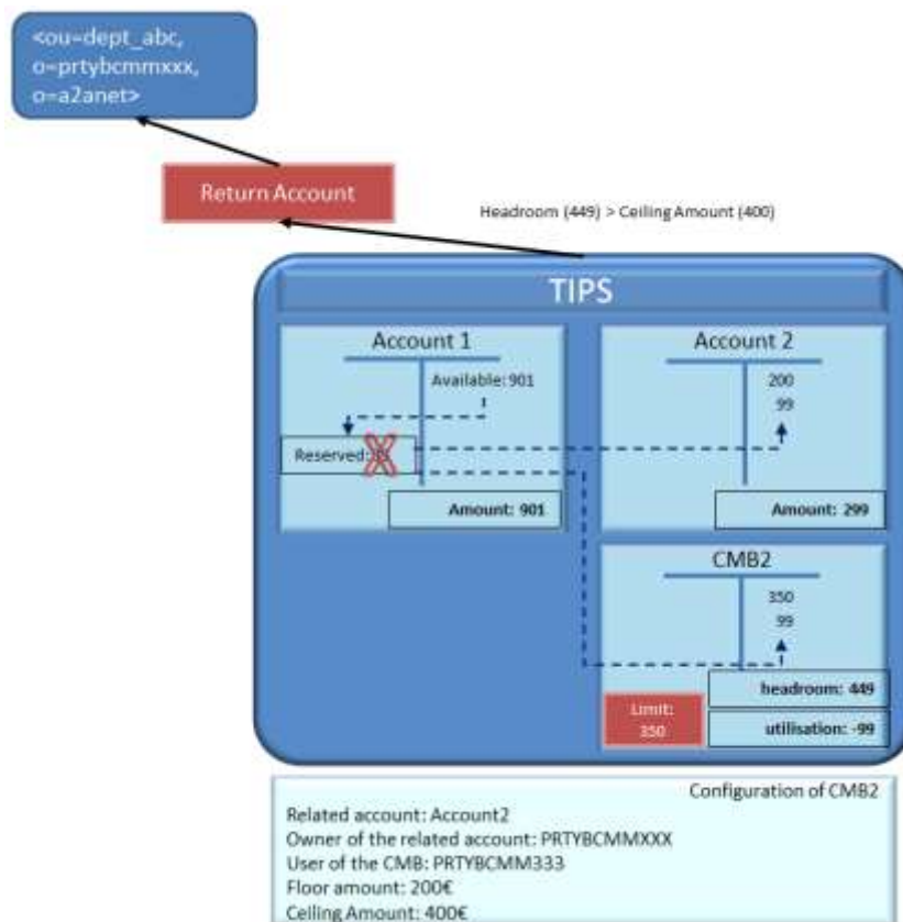
Figure 251247227 – Ceiling notification settlement
