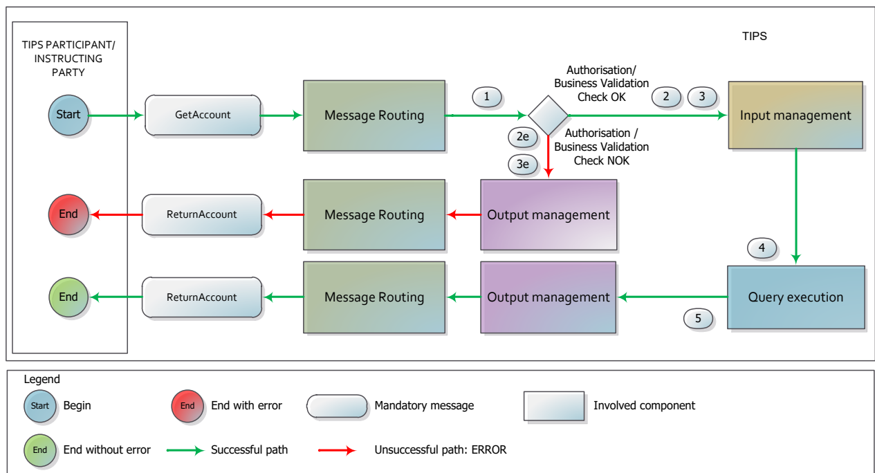
Figure 253249229 – Account Balance Status query flow
