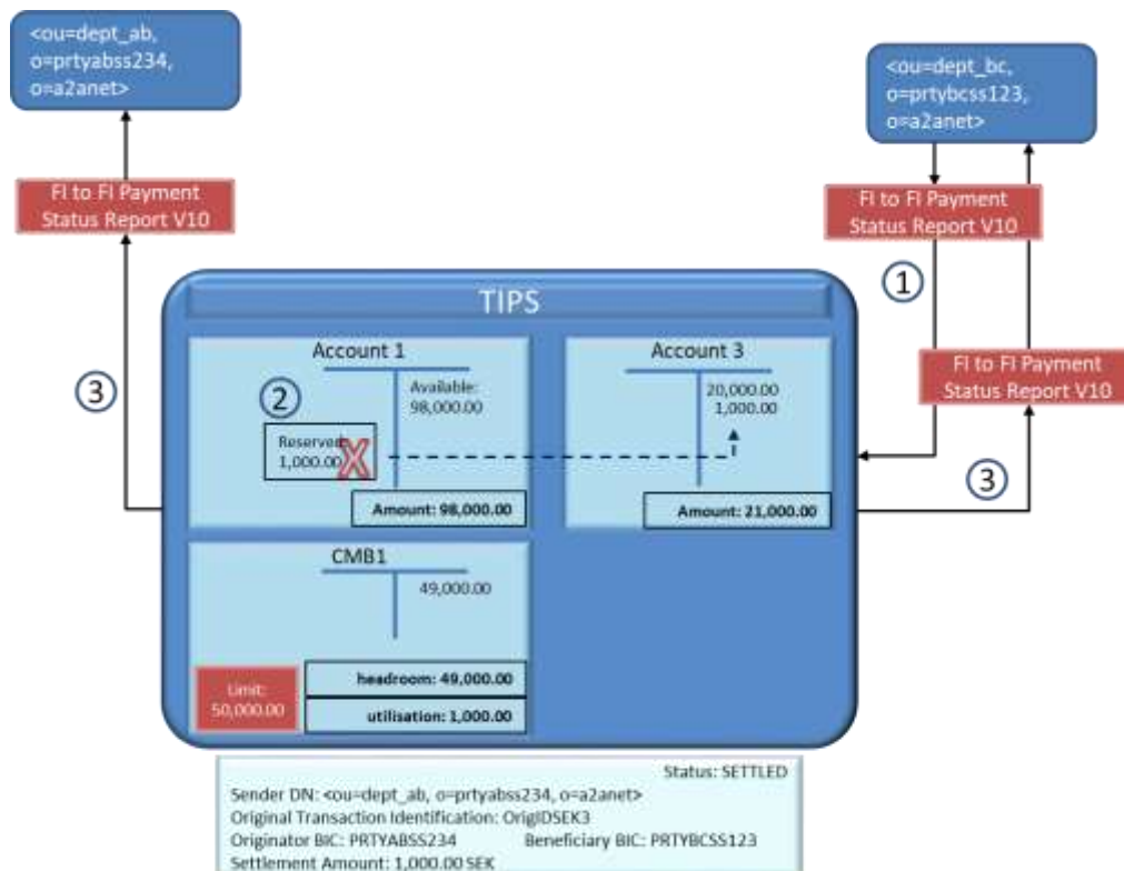
Figure 737373 – Successful Instant Payment transaction: settlement phase
