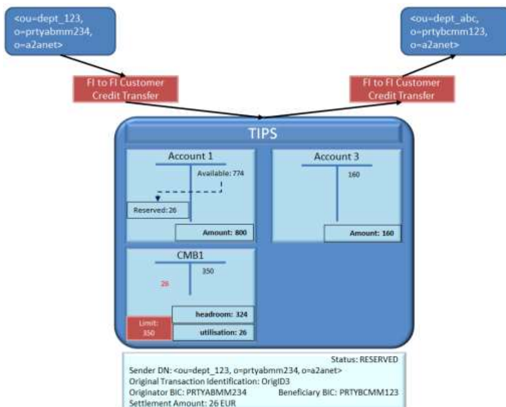
Figure 303030 – Successful Instant Payment transaction: reservation of funds
