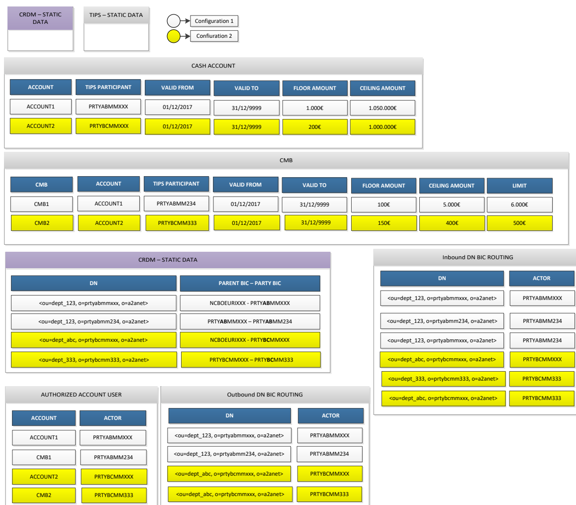
Figure 200196180 – Transaction status investigation examples: data constellation
