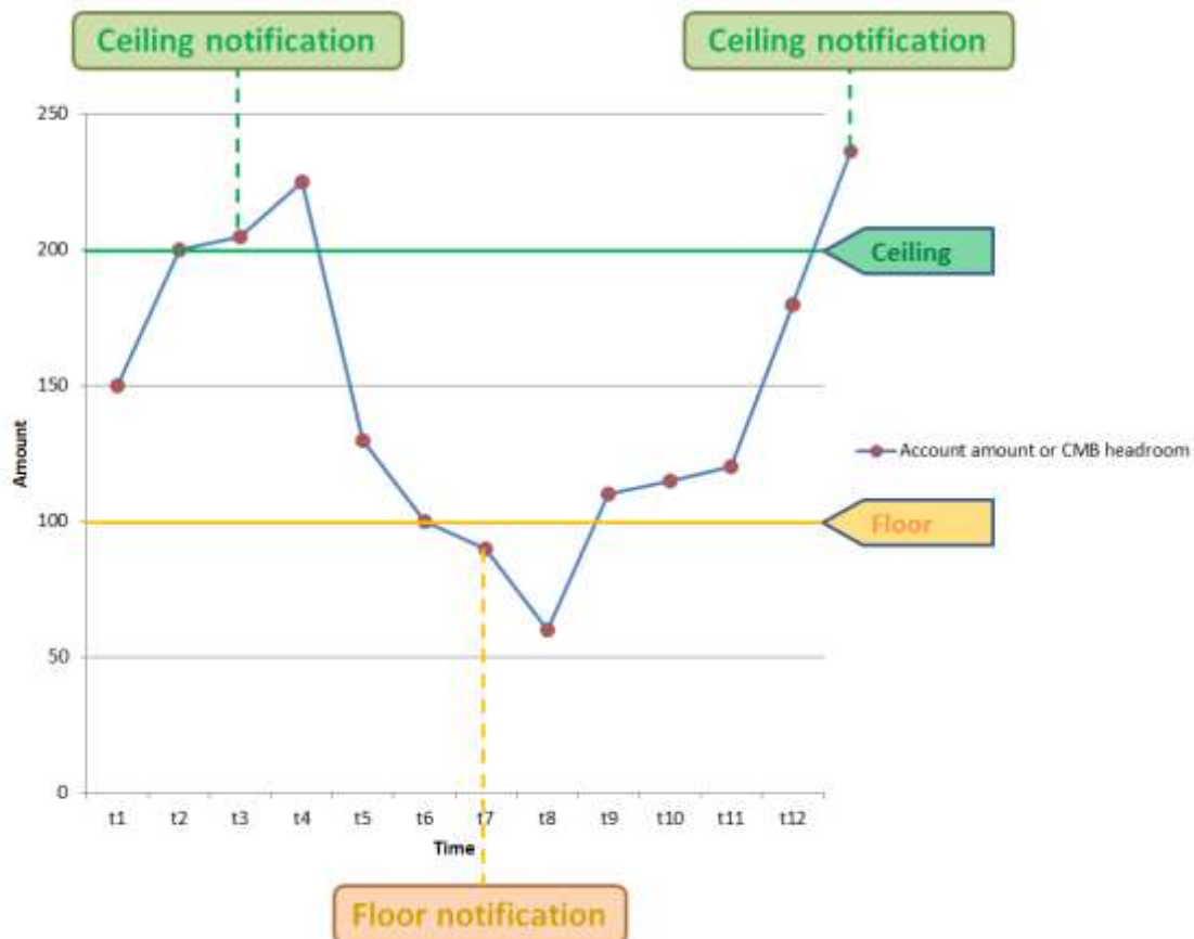
Figure 248244224 – Floor and ceiling notification triggers
