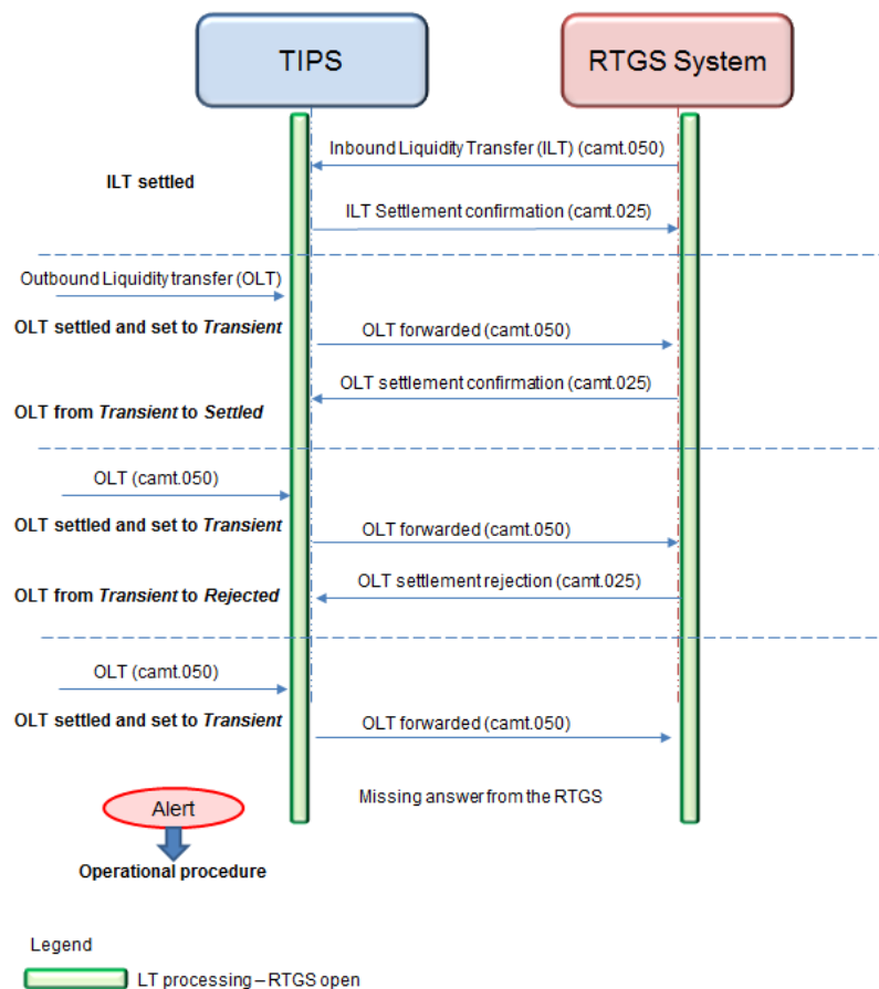
Figure 161616 – Interaction with RTGS System for Liquidity Transfers
