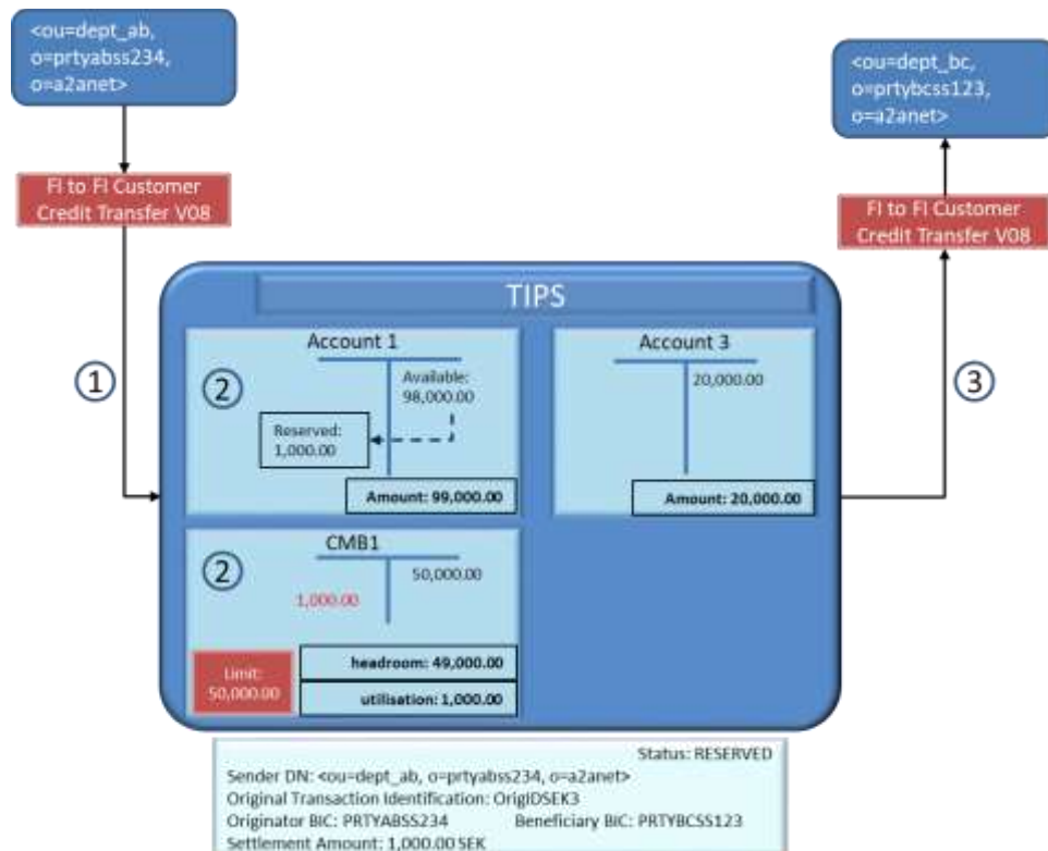
Figure 717474 – Successful Instant Payment transaction: reservation of funds
