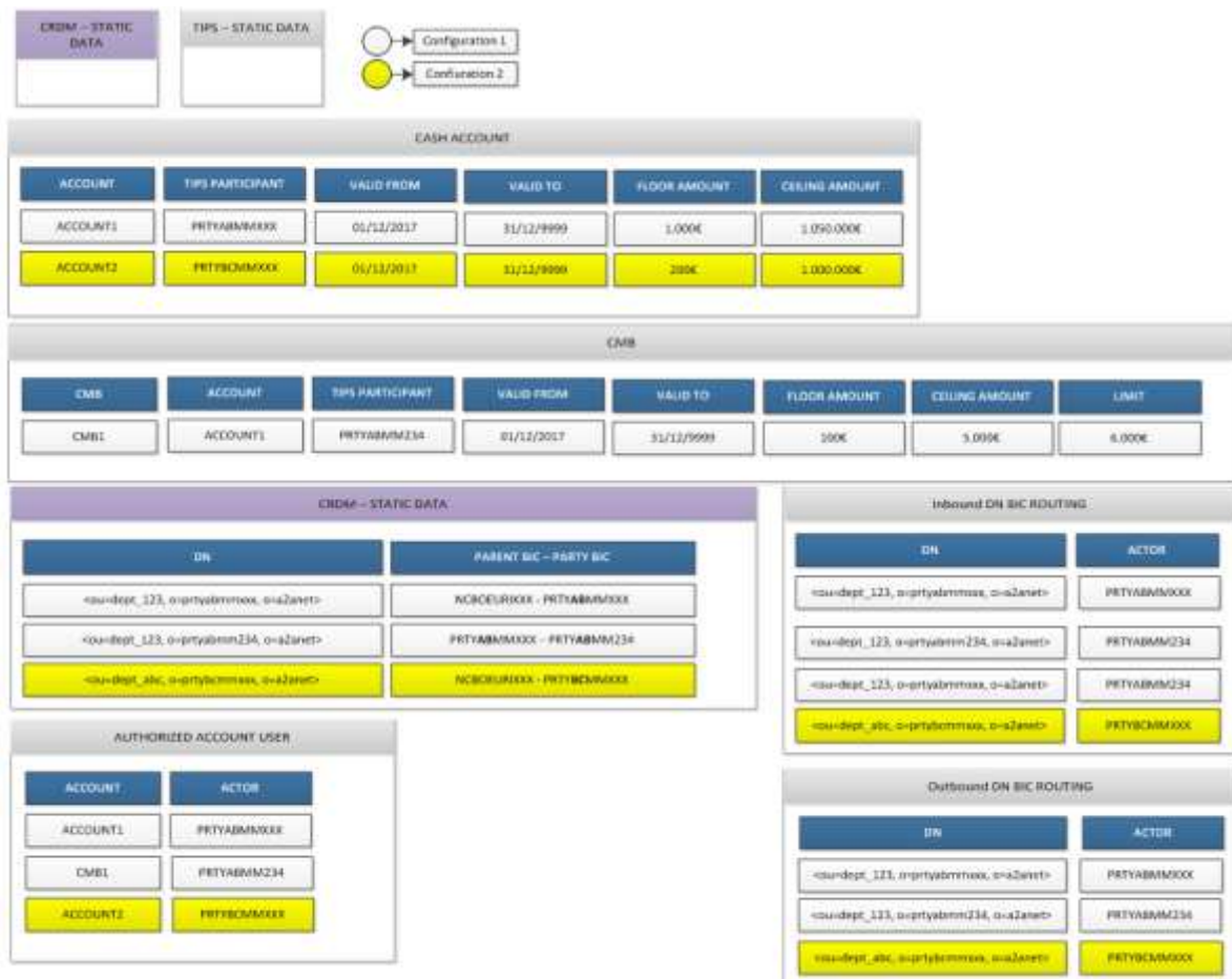
Figure 255251231 – Queries examples: data constellation
