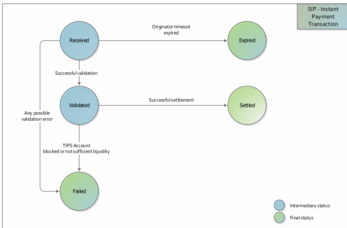
Figure 888 – SIP Instant Payment Transaction status transition diagram
