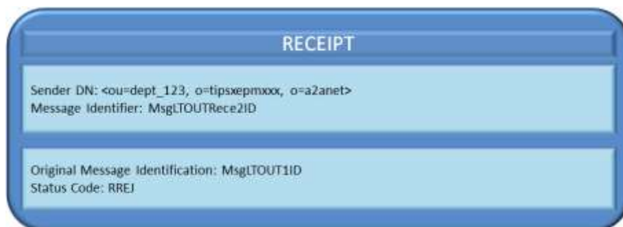
Figure 235231211 – Outbound Liquidity Transfer order: negative Receipt sent by TIPS
