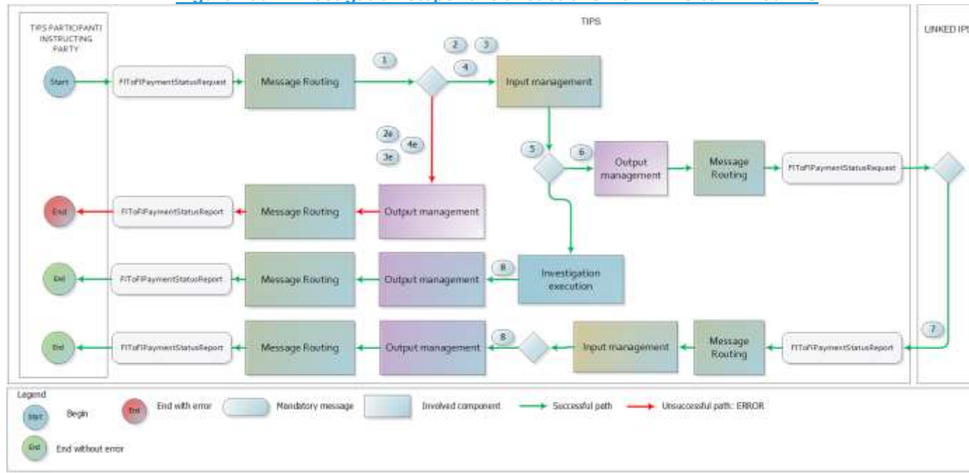
Figure 199 - Investigation steps for transactions from TIPS to Linked IPS
