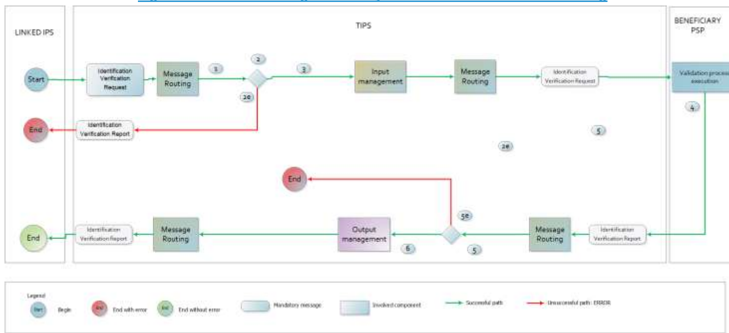
Figure 163 - TIPS incoming Instant Payment validation flow for interlinking
