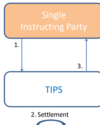
Figure 777 – Single Instructing Party settlement model for Instant Payments
