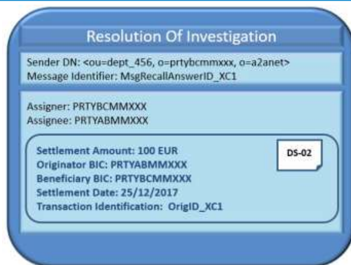
Figure 192190 - ResolutionOfInvestigation – Negative Response
