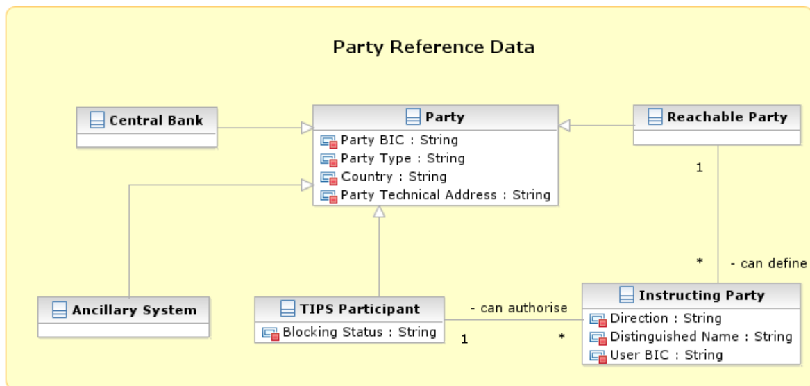
Figure 333 – Party reference data model
