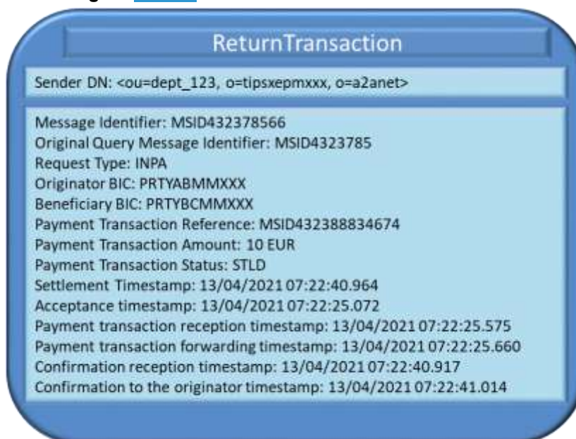
Figure 264260240 – Successful ReturnTransaction
