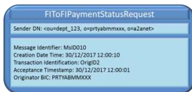
Figure 203199183 – Unsuccessful FIToFIPaymentStatusRequest
