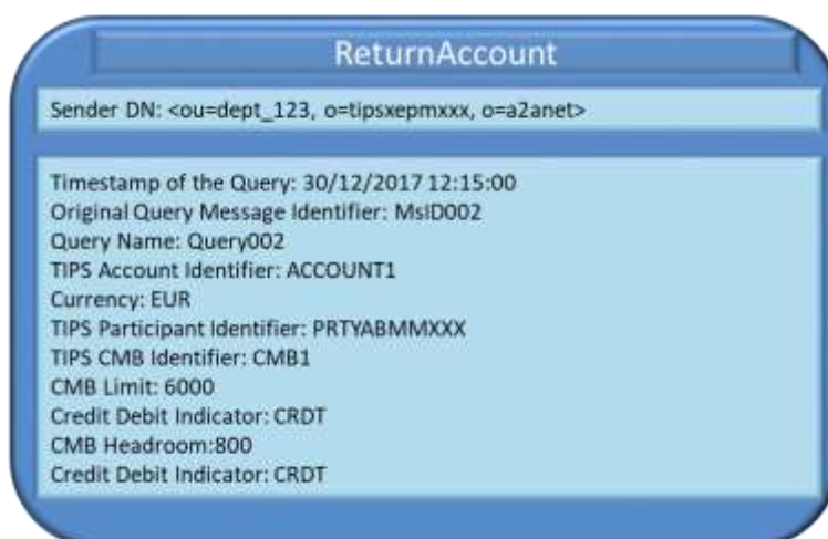
Figure 259255235 – Successful ReturnAccount
