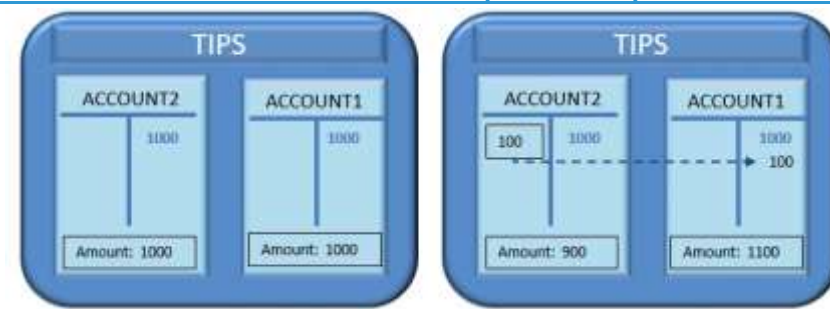
Figure 188186 - Recall XCY successful scenario: positive response – Settlement Process
