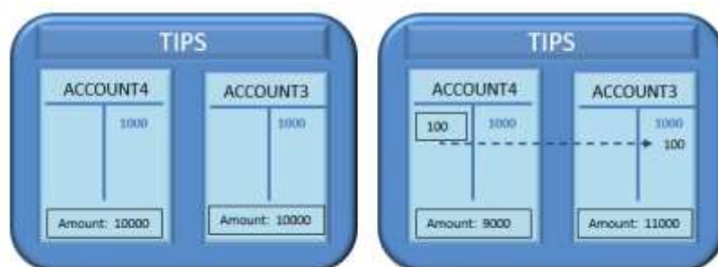
Figure 191489 - Recall XCY successful scenario: positive response – Settlement Process
