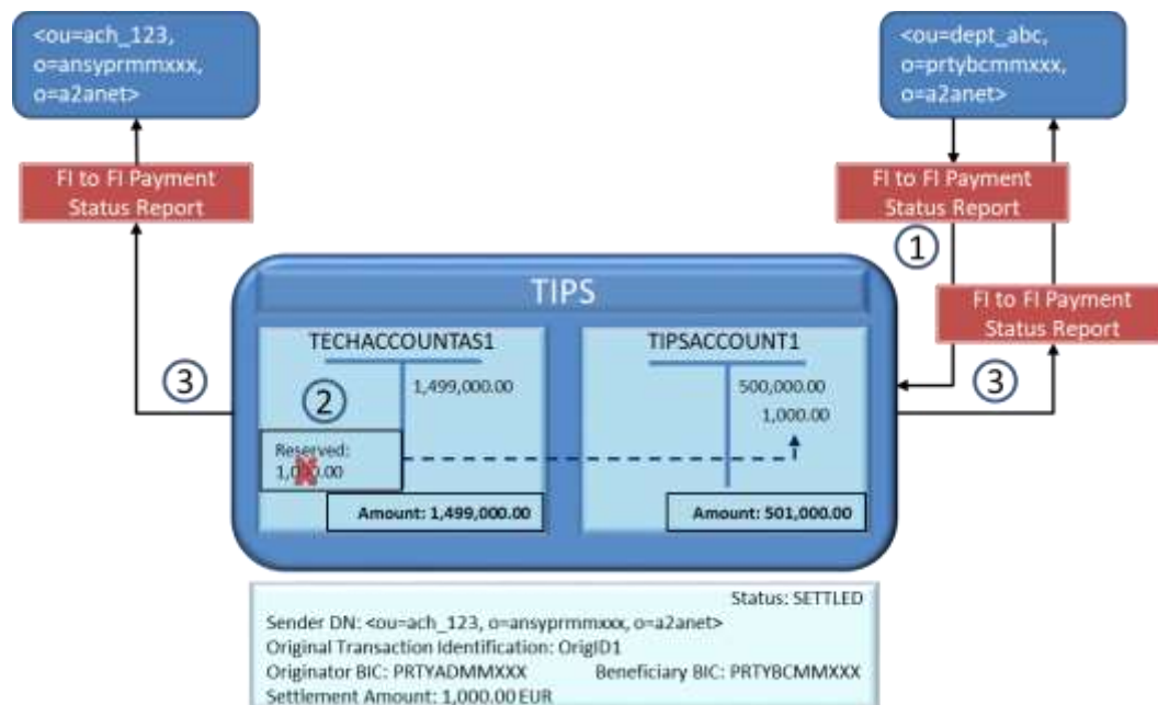
Figure 444444 – Successful Instant Payment transaction successful: settlement phase
