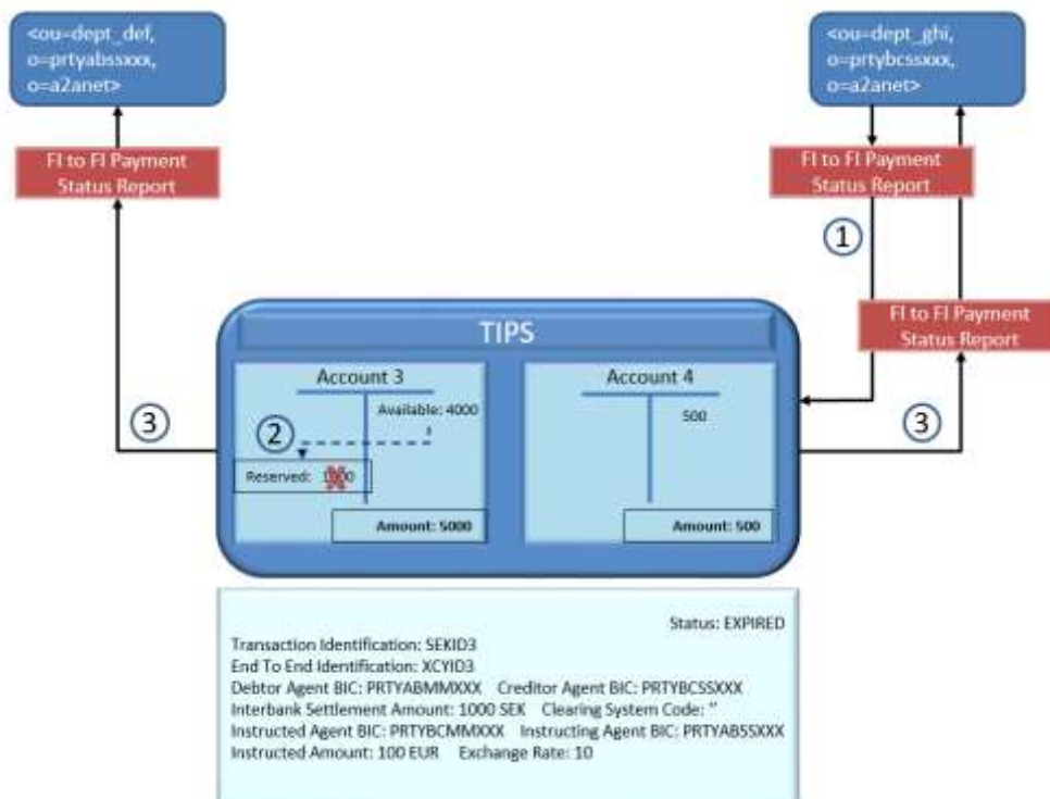
Figure 159159159 – Beneficiary side timeout error: release of funds in the destination currency
