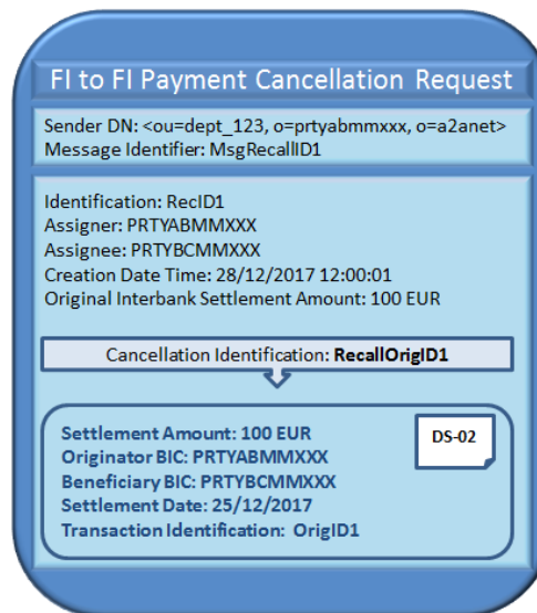
Figure 168166164 – Recall successful scenario: positive response – FItoFIPaymentCancellationRequest
