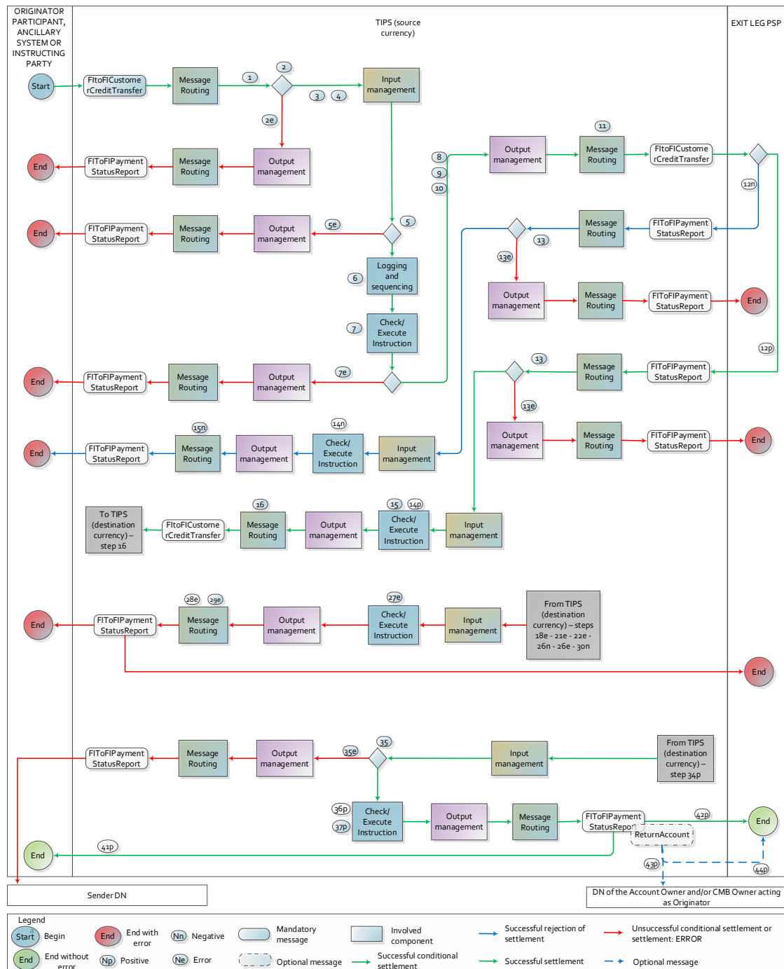
Figure 140140140 – Instant Payment transaction flow for cross-currency LKTELKT settlement model (part I)
