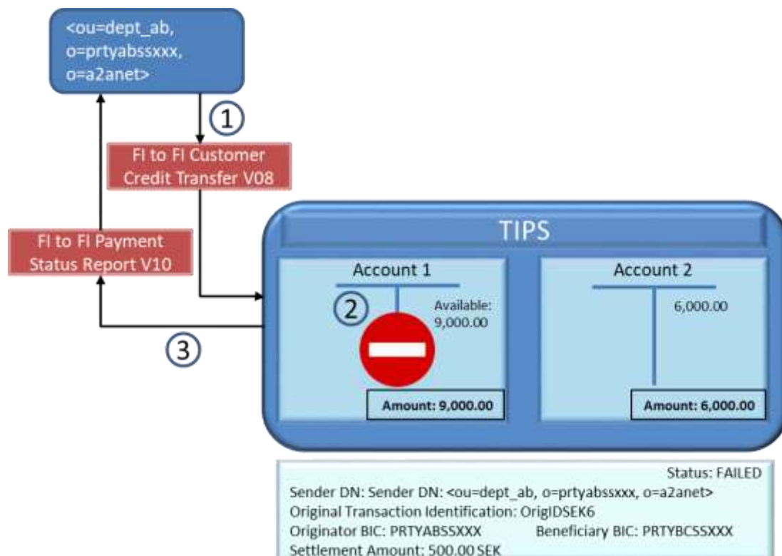
Figure 868686 – Blocked account error: transaction failed
