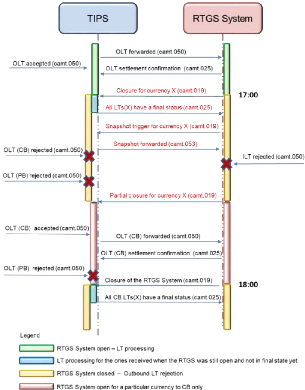
Figure 191919 – Snapshot generation and partial closure status
