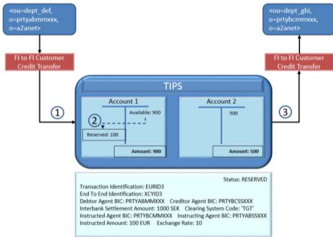
Figure 155155155 – Beneficiary side timeout: reservation of funds in the source currency
