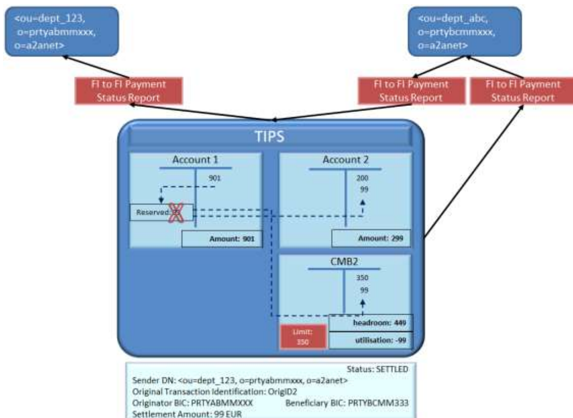
Figure 363636 – Successful Instant Payment transaction: settlement phase
