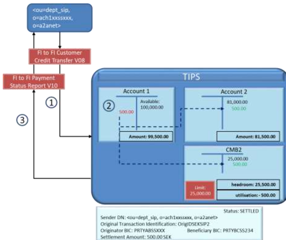
Figure 113113113 – Successful Instant Payment in non-Euro currency with SIP: settlement phase
