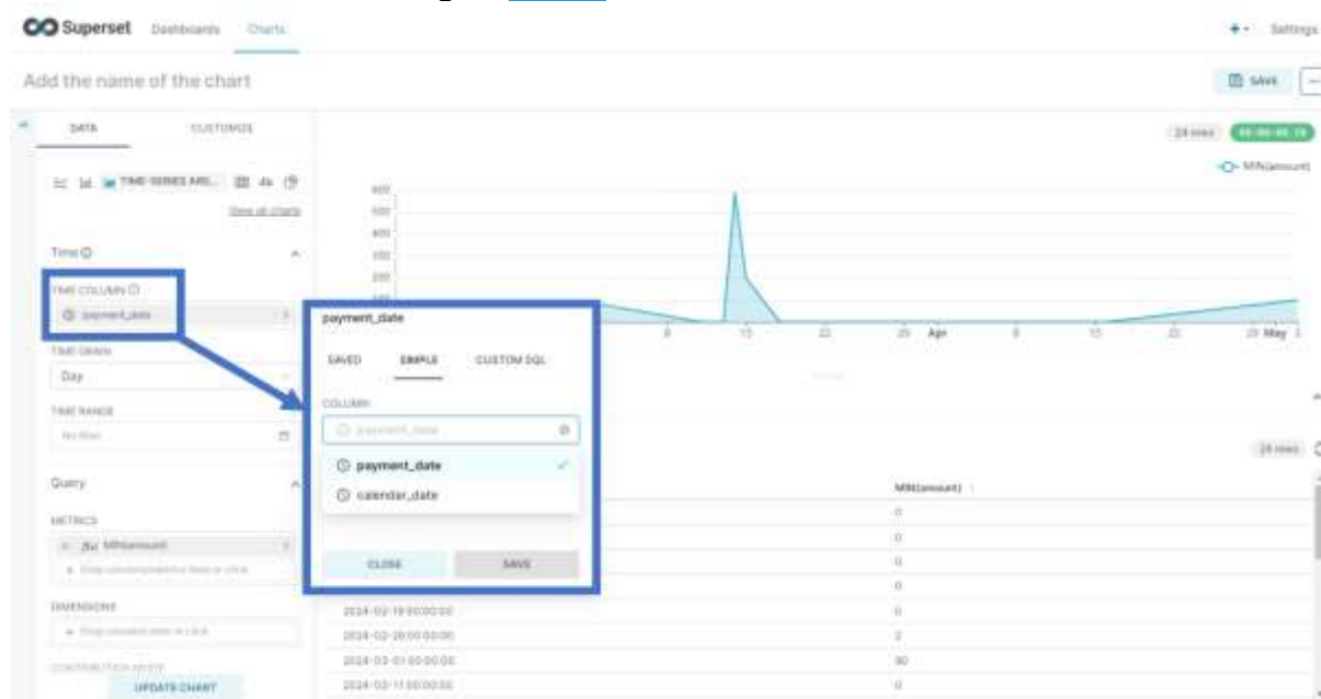
Figure 310 306 286 – Time column field
