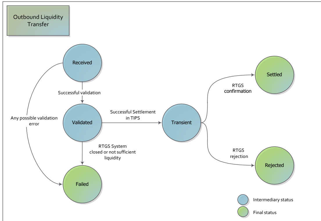
Figure 11111 – Outbound Liquidity Transfer status diagram
