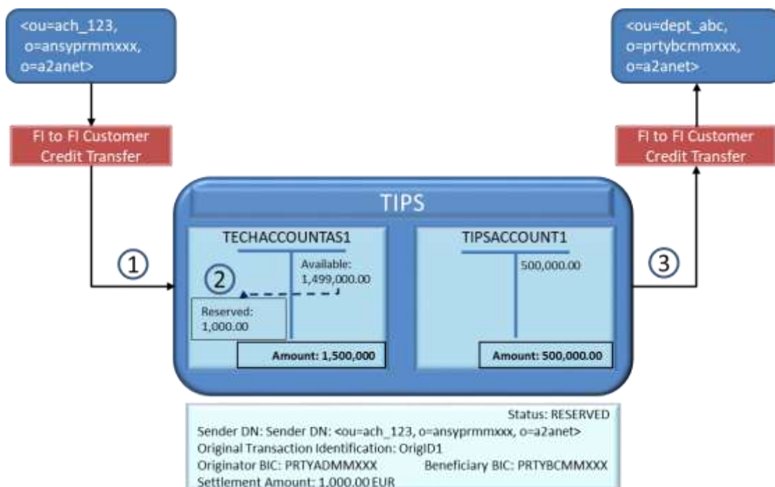
Figure 424242 – Successful Instant Payment transaction: reservation of funds
