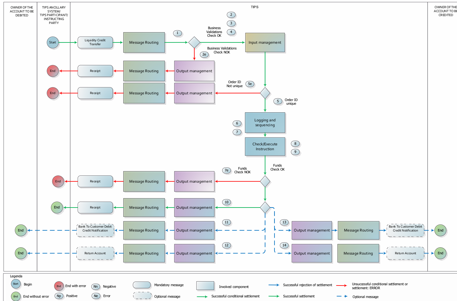
Figure 237233243 – Intra-service Liquidity Transfer diagram
