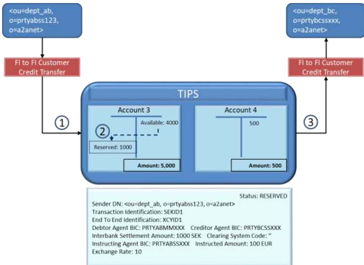
Figure 129129129 – Successful Instant Payment transaction: reservation of funds
