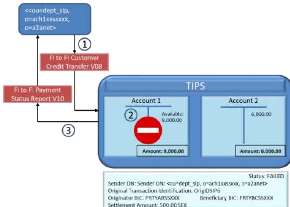
Figure 119119119 – Blocked account error: transaction failed
