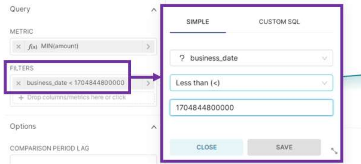
Figure 314310290 – Business date filtering
