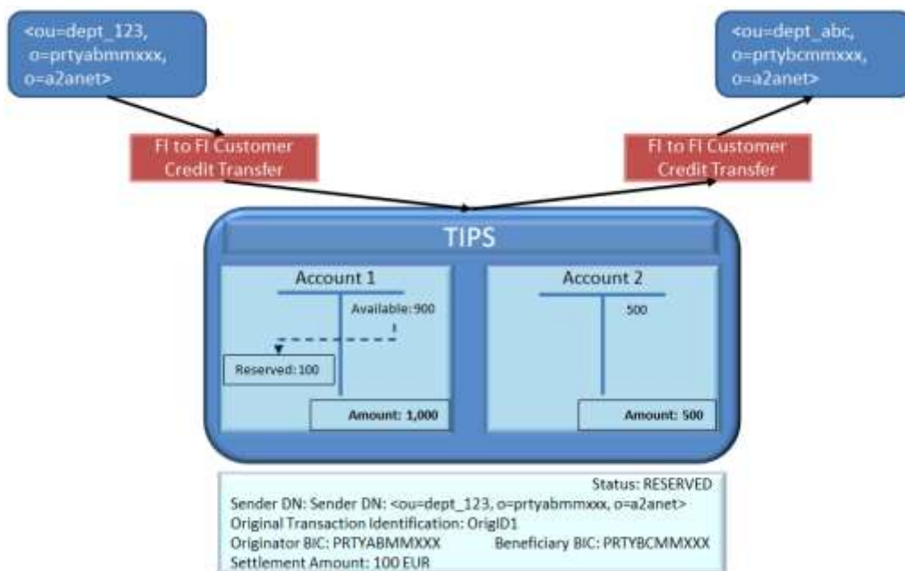
Figure 262626 – Successful Instant Payment transaction: reservation of funds
