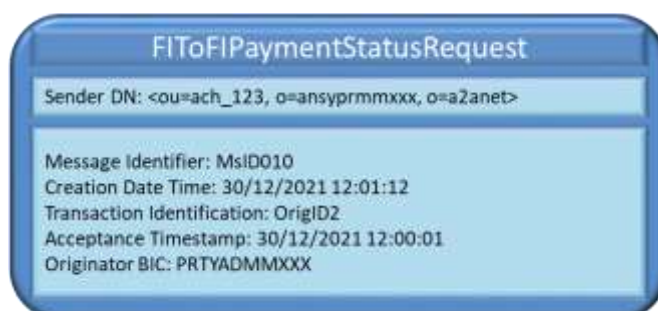
Figure 205201485 – Successful FIToFIPaymentStatusRequest originated by an AS
