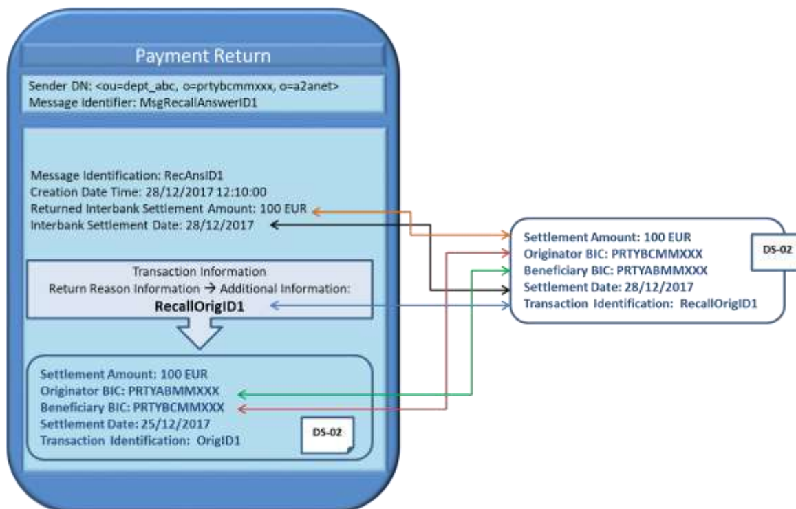
Figure 170168166 – Recall successful scenario: positive response – Recall Dataset
