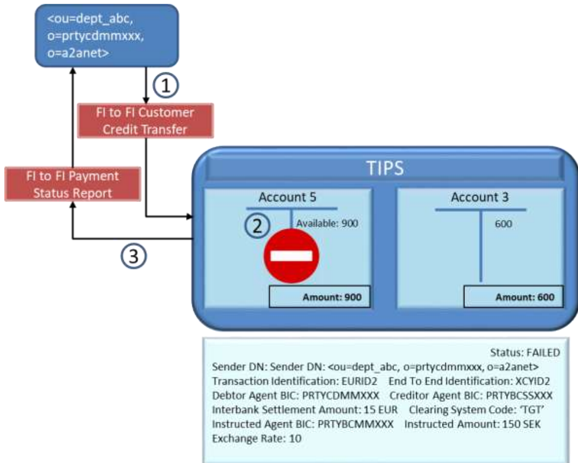
Figure 133133133 – Blocked account error: transaction failed
