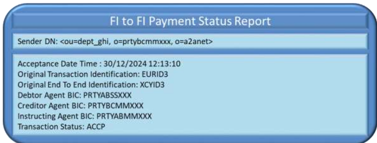
Figure 137137137 – Beneficiary side timeout error: FltoFIPaymentStatusReport
