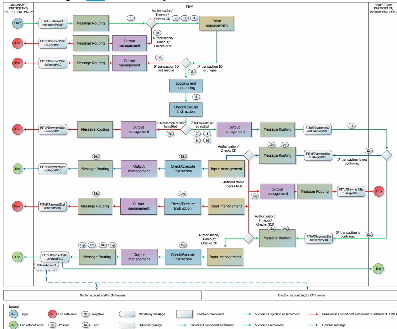
Figure 636363 – Instant Payment transaction flow for non-Euro currencies
