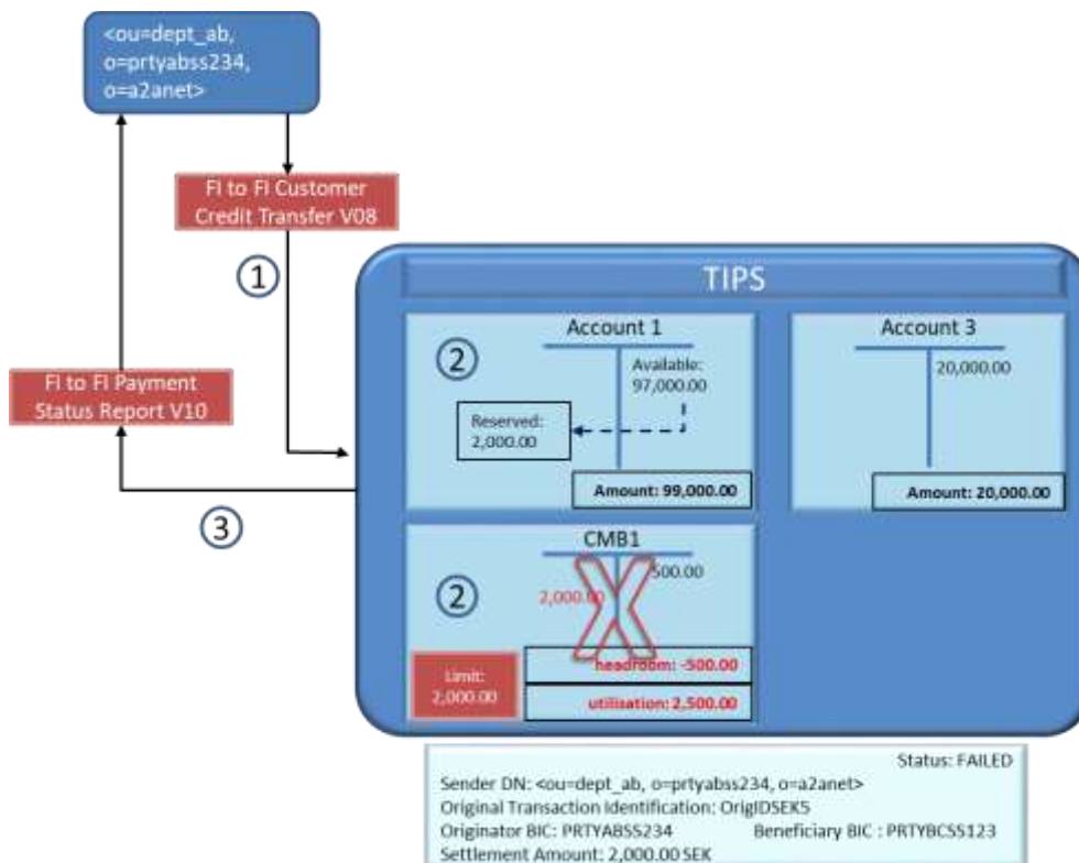
Figure 838383 – Headroom error: transaction failed
