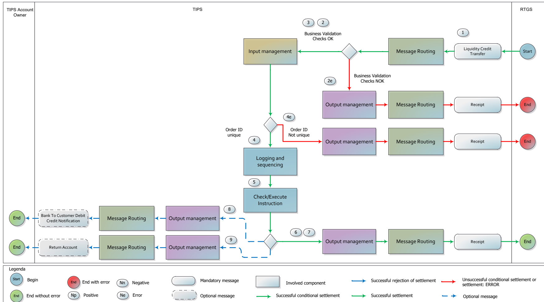
Figure 211207187 – Inbound Liquidity Transfer Order flow
