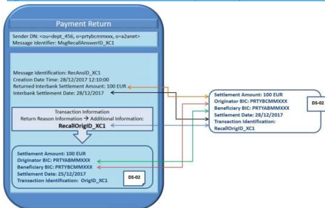
Figure 187485 - Recall XCY successful scenario: positive response – Recall Dataset
