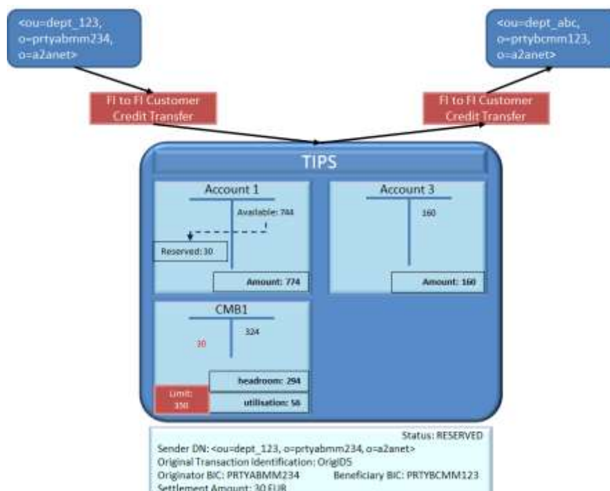
Figure 525252 – Beneficiary side timeout error: reservation of funds
