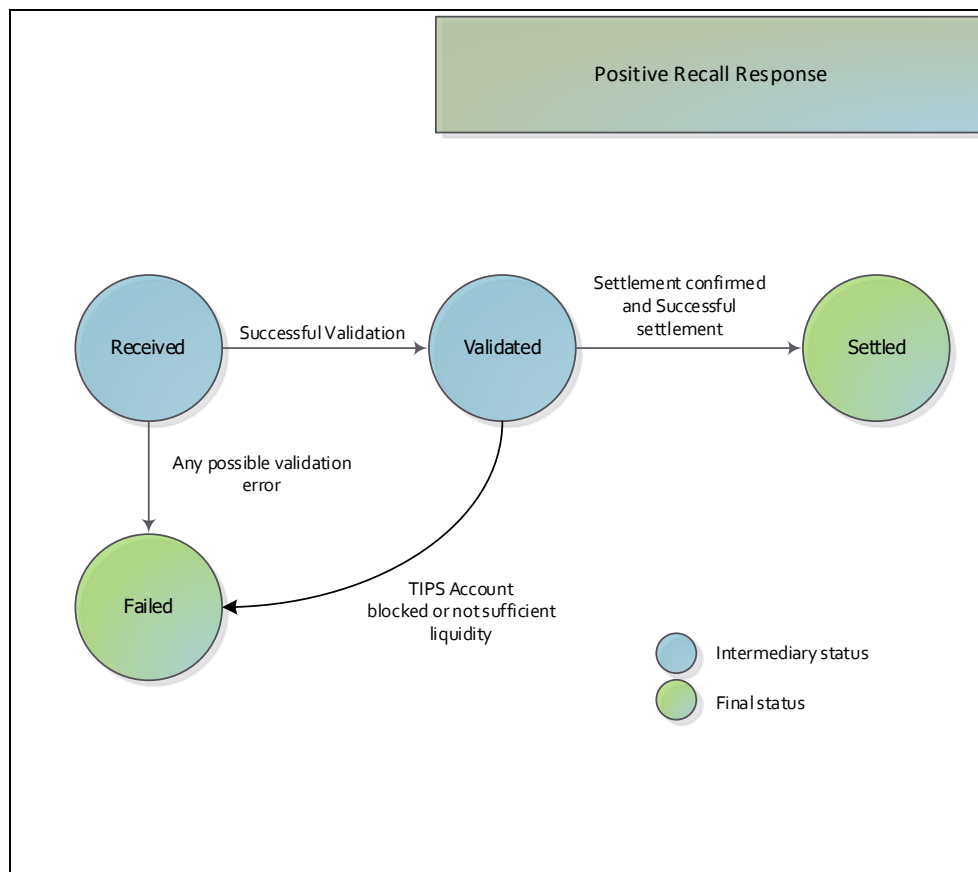
Figure 999 – Positive Recall Response status diagram
