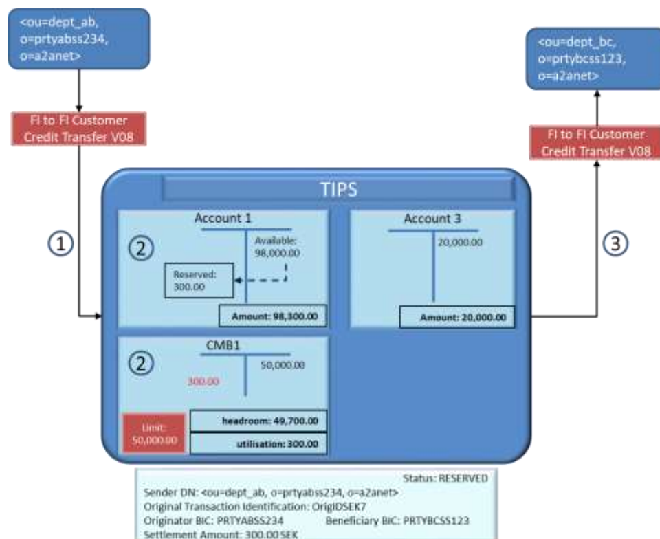
Figure 898989 – Beneficiary side timeout error: reservation of funds
