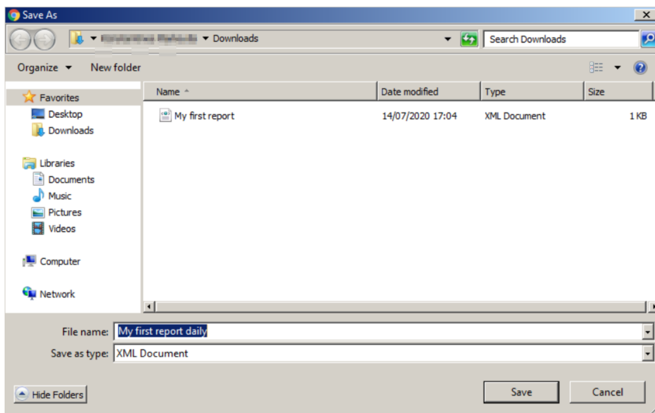
Figure 90: Save Report
