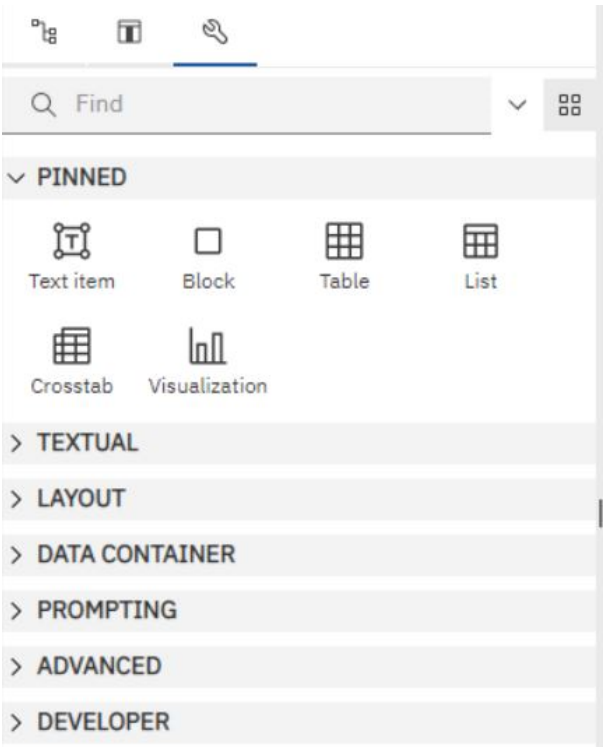
Figure 468: Toolbox bar
